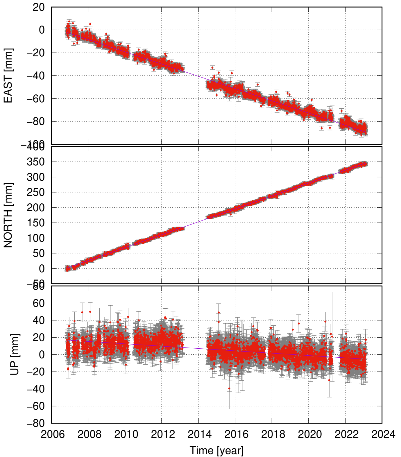
KVIS (66.10, -17.27) time series (ITRF 2014) v_e = -5.36 \pm 0.15 ; v_n = 21.16 \pm 0.15 ; v_u = -1.37 \pm 0.45 mm/yr
