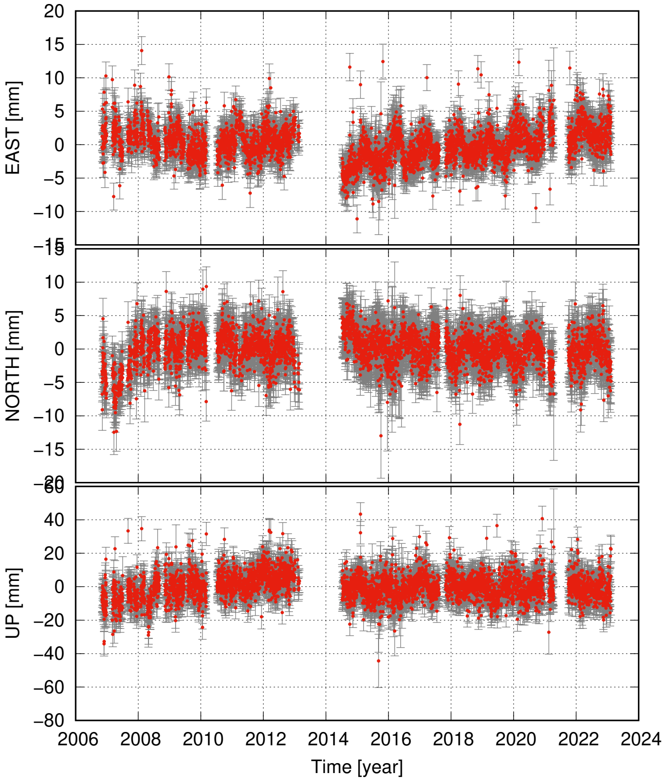
KVIS residual time series (some major events removed as well)
