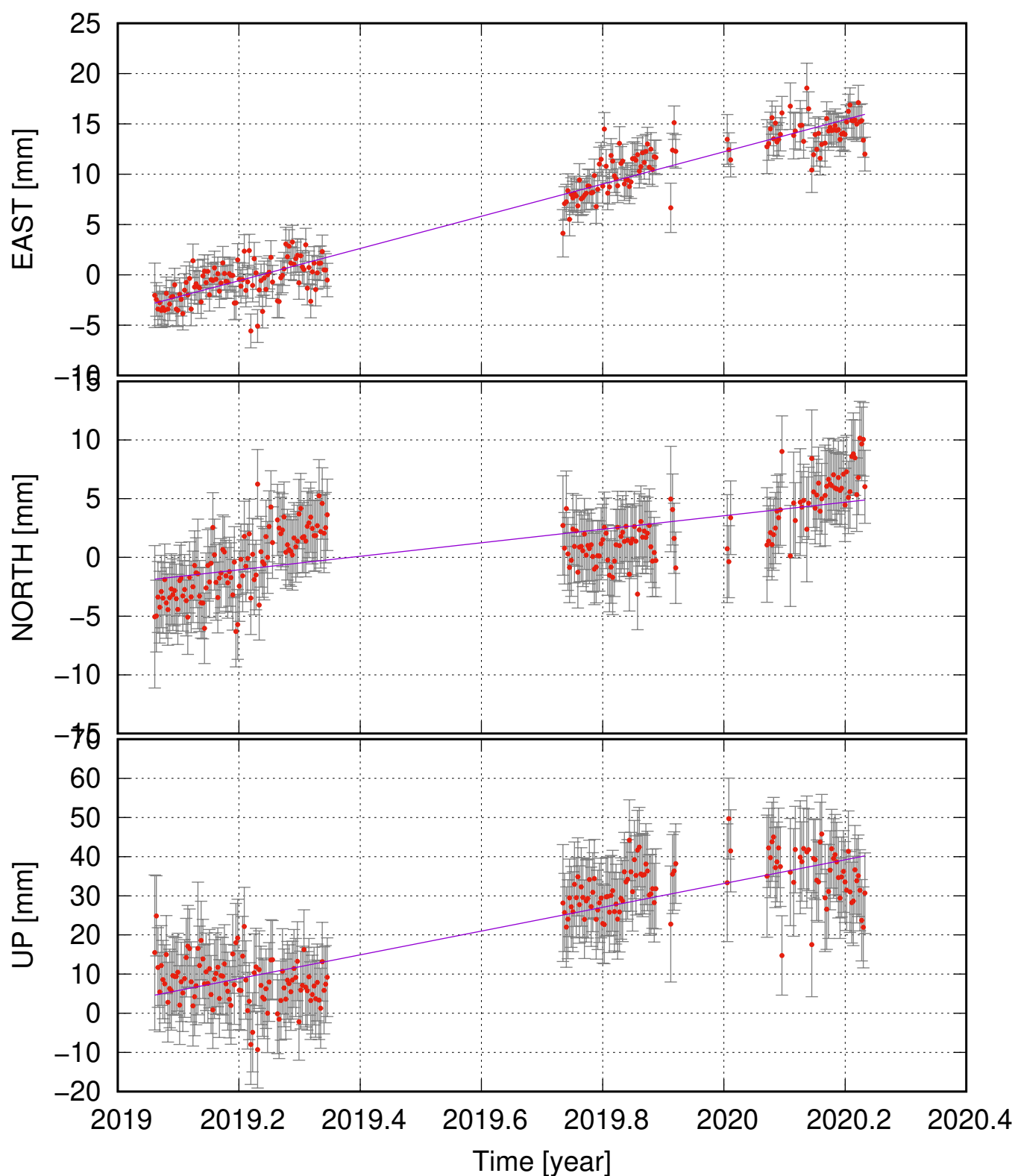
KVIC (63.93, -16.50) time series (ITRF 2014) v_e = 16.01 \pm 1.40 ; v_n = 5.75 \pm 2.02 ; v_u = 30.32 \pm 5.84 mm/yr
