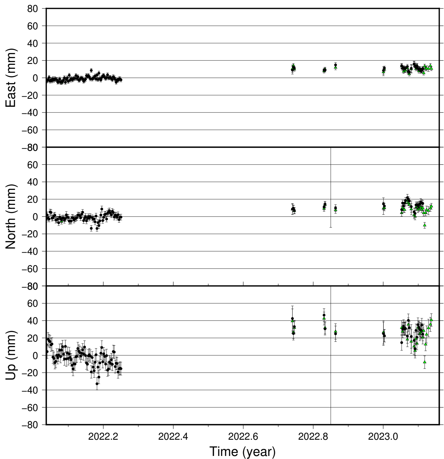
KVEC time series (IGS 2014), last 400 days
