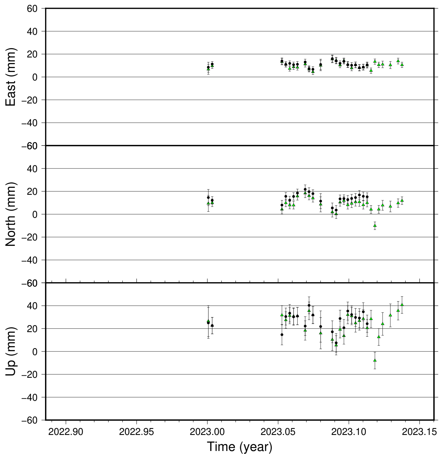
KVEC time series (IGS 2014), last 100 days
