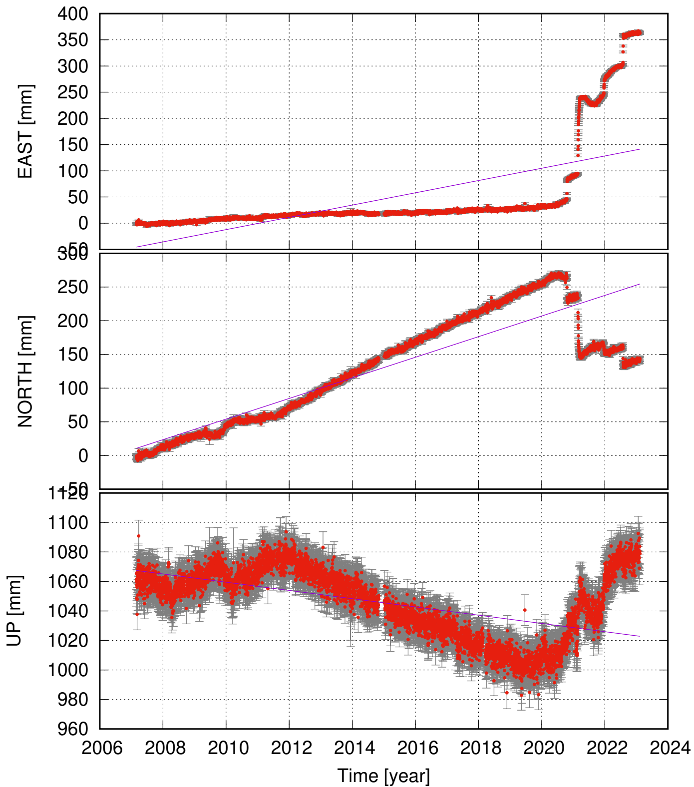
KRIV (63.88, -22.08) time series (ITRF 2014) v_e = 11.72 \pm 4.32 ; v_n = 15.28 \pm 2.49 ; v_u = -2.79 \pm 1.27 mm/yr
