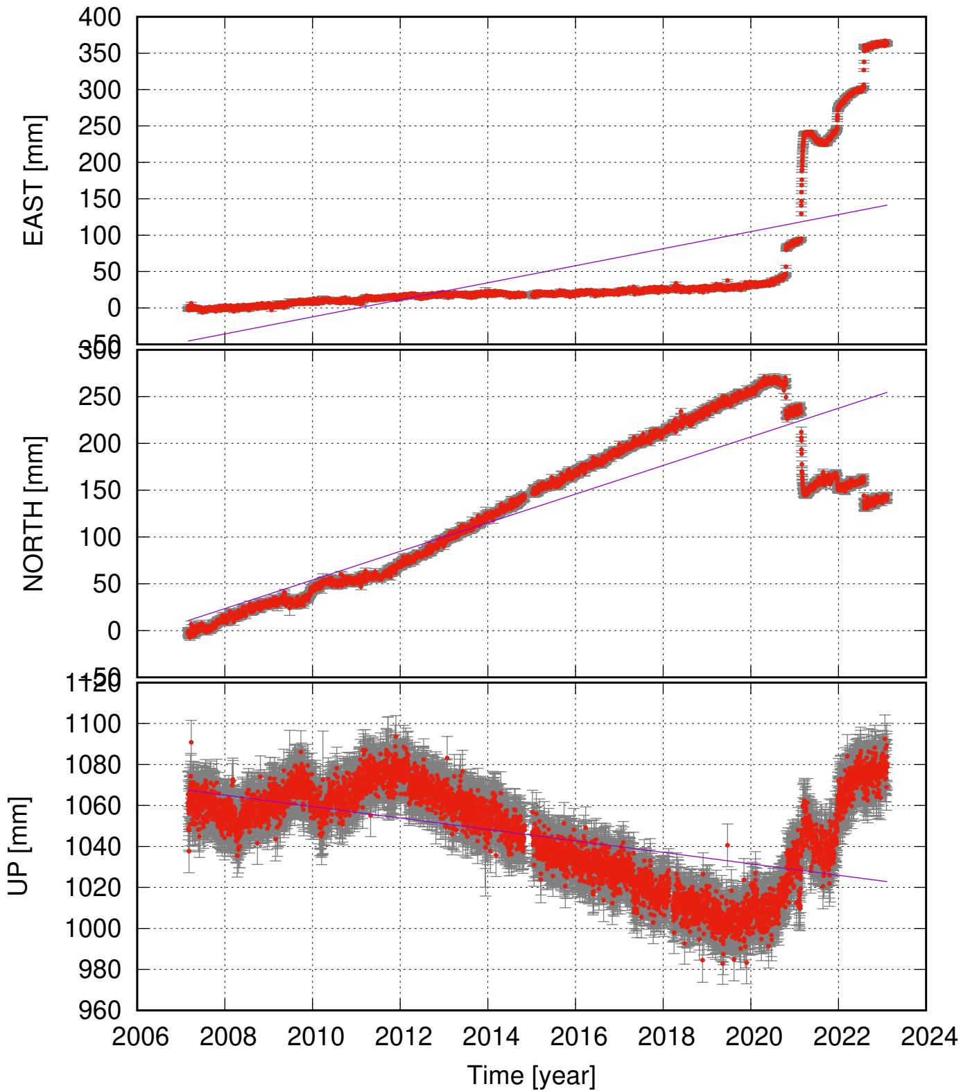
KRIV (63.88, -22.08) time series (ITRF 2014) v_e = 11.72 \pm 4.32 ; v_n = 15.28 \pm 2.49 ; v_u = -2.79 \pm 1.27 mm/yr
