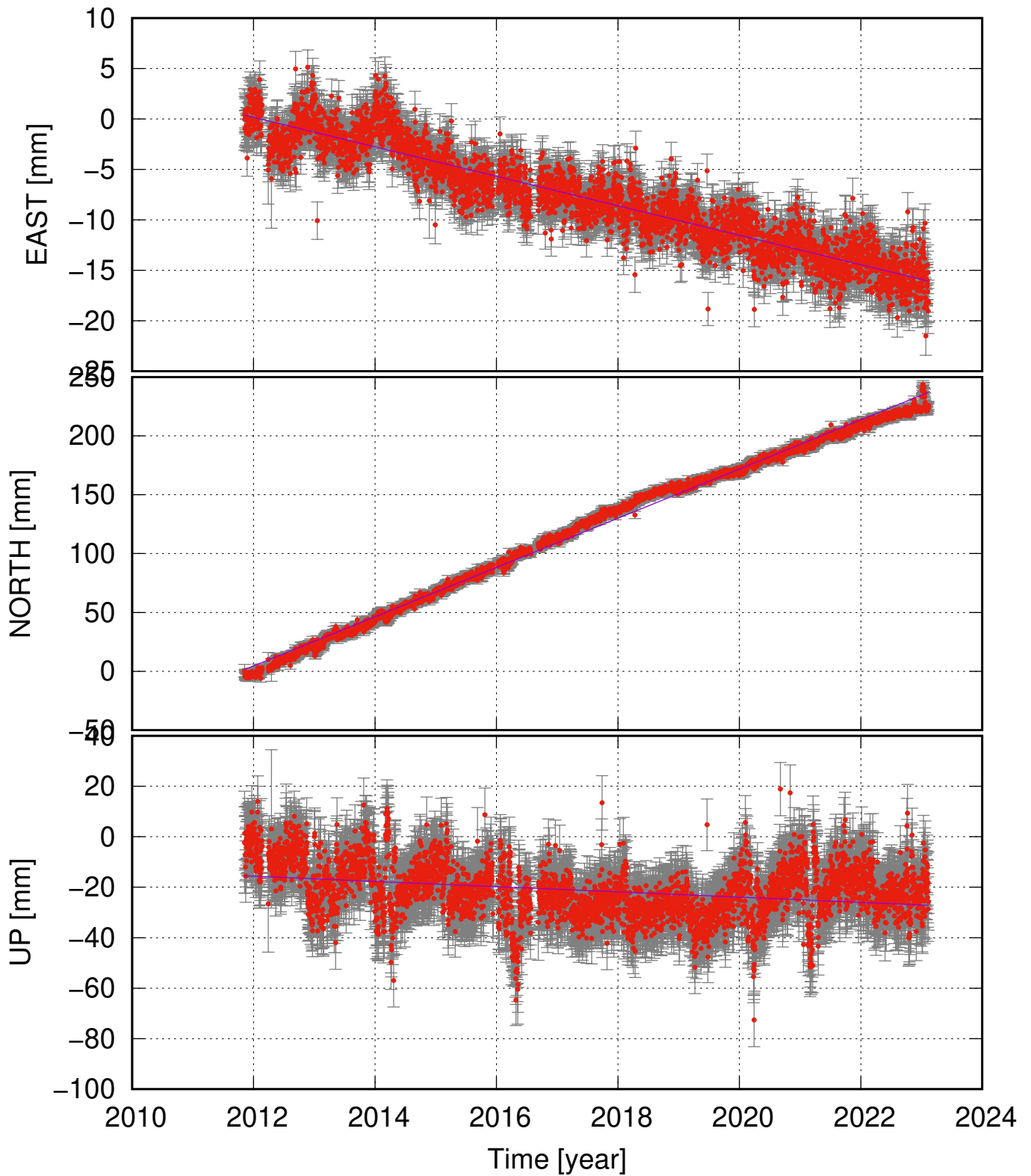
KRAC (65.69, -16.77) time series (ITRF 2014) v_e = -1.46 \pm 0.16 ; v_n = 20.91 \pm 0.45 ; v_u = -1.04 \pm 0.88 mm/yr
