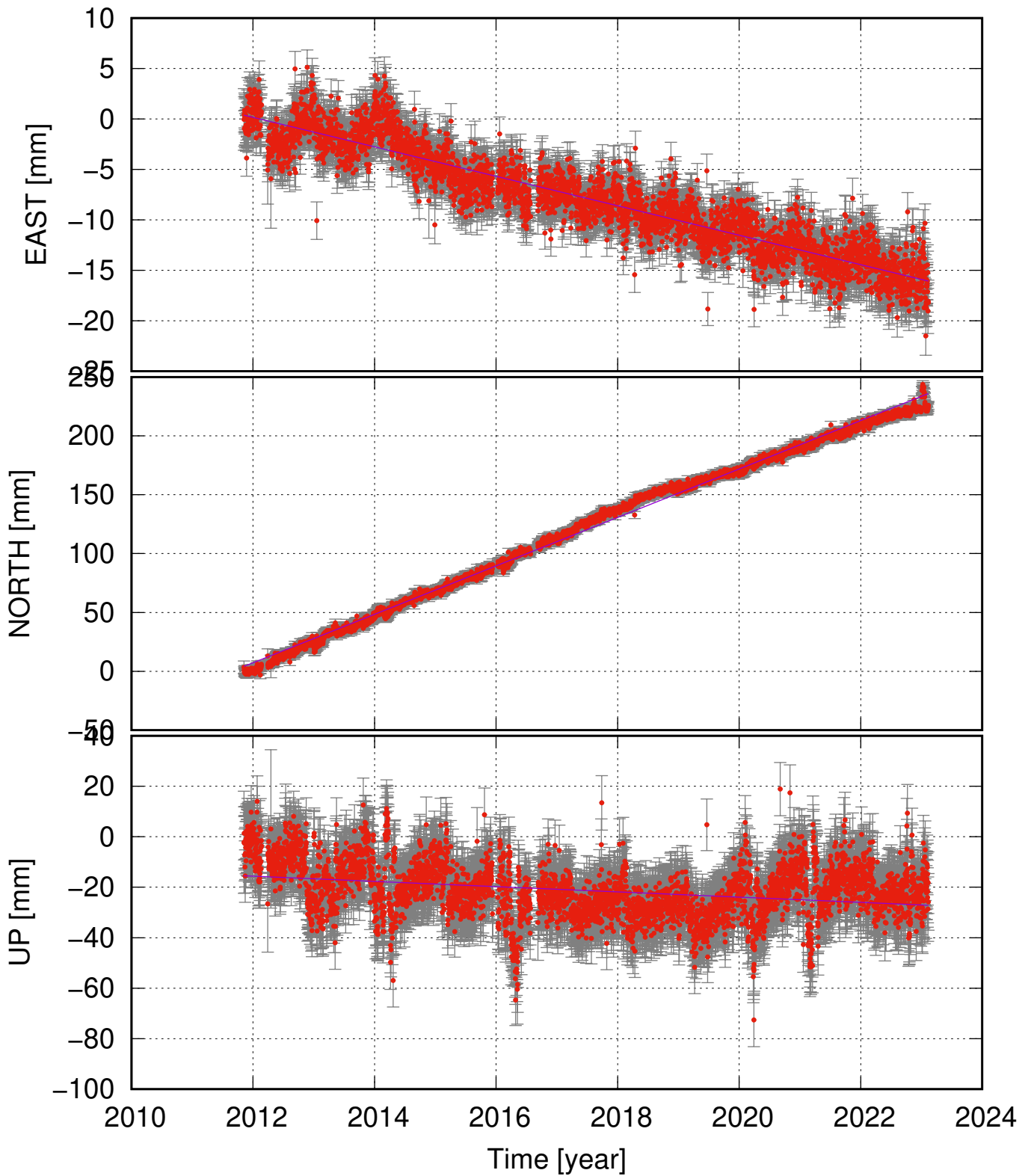
KRAC (65.69, -16.77) time series (ITRF 2014) v_e = -1.46 \pm 0.16 ; v_n = 20.59 \pm 0.41 ; v_u = -1.04 \pm 0.88 mm/yr
