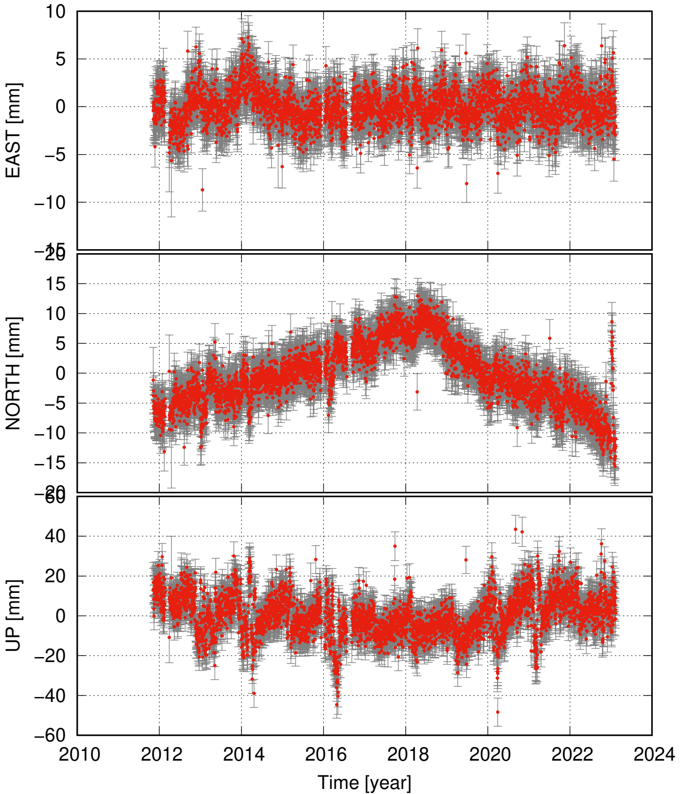
KRAC residual time series (some major events removed as well)
