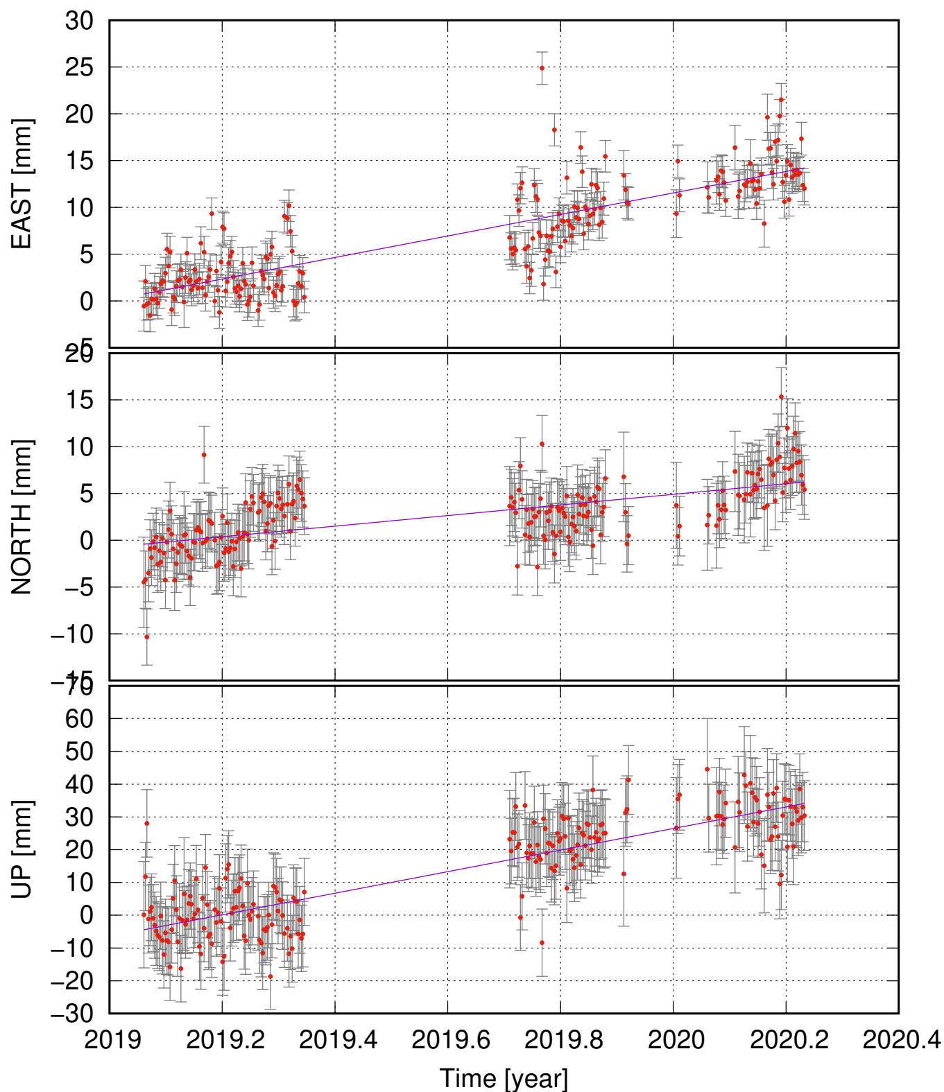
KOTC (63.93, -16.76) time series (ITRF 2014) v_e = 11.48 \pm 2.44 ; v_n = 5.67 \pm 2.26 ; v_u = 32.92 \pm 6.90 mm/yr
