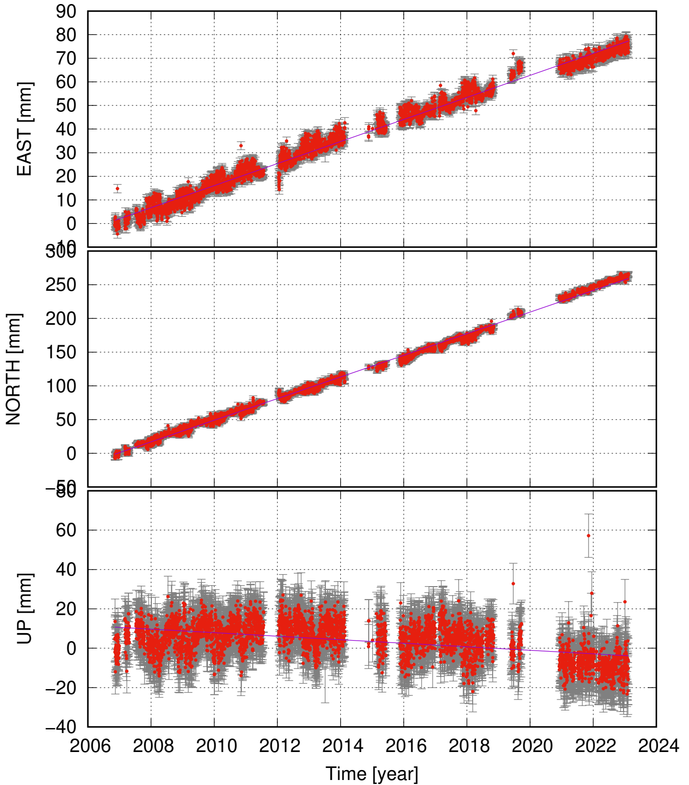
KOSK (66.30, -16.44) time series (ITRF 2014) v_e = 4.67 \pm 0.16 ; v_n = 16.04 \pm 0.26 ; v_u = -0.90 \pm 0.47 mm/yr
