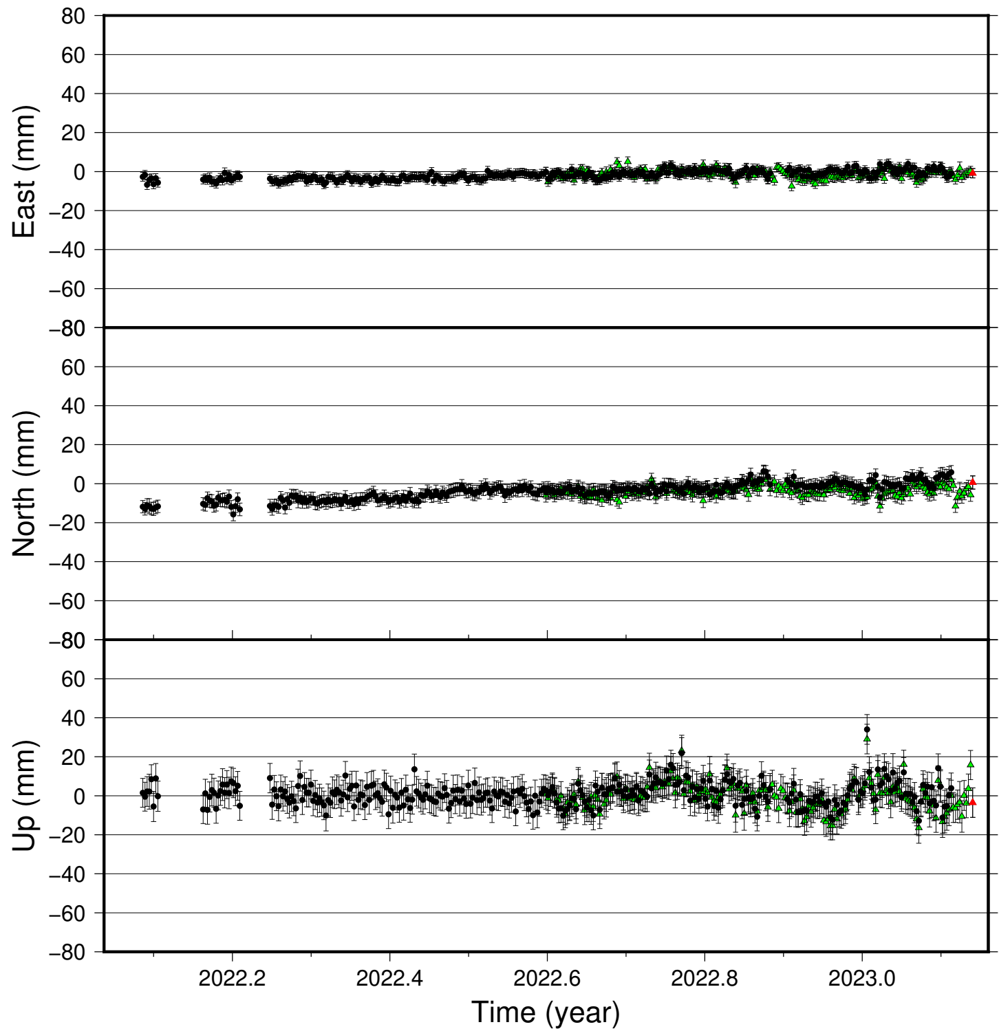
KOSK time series (IGS 2014), last 400 days
