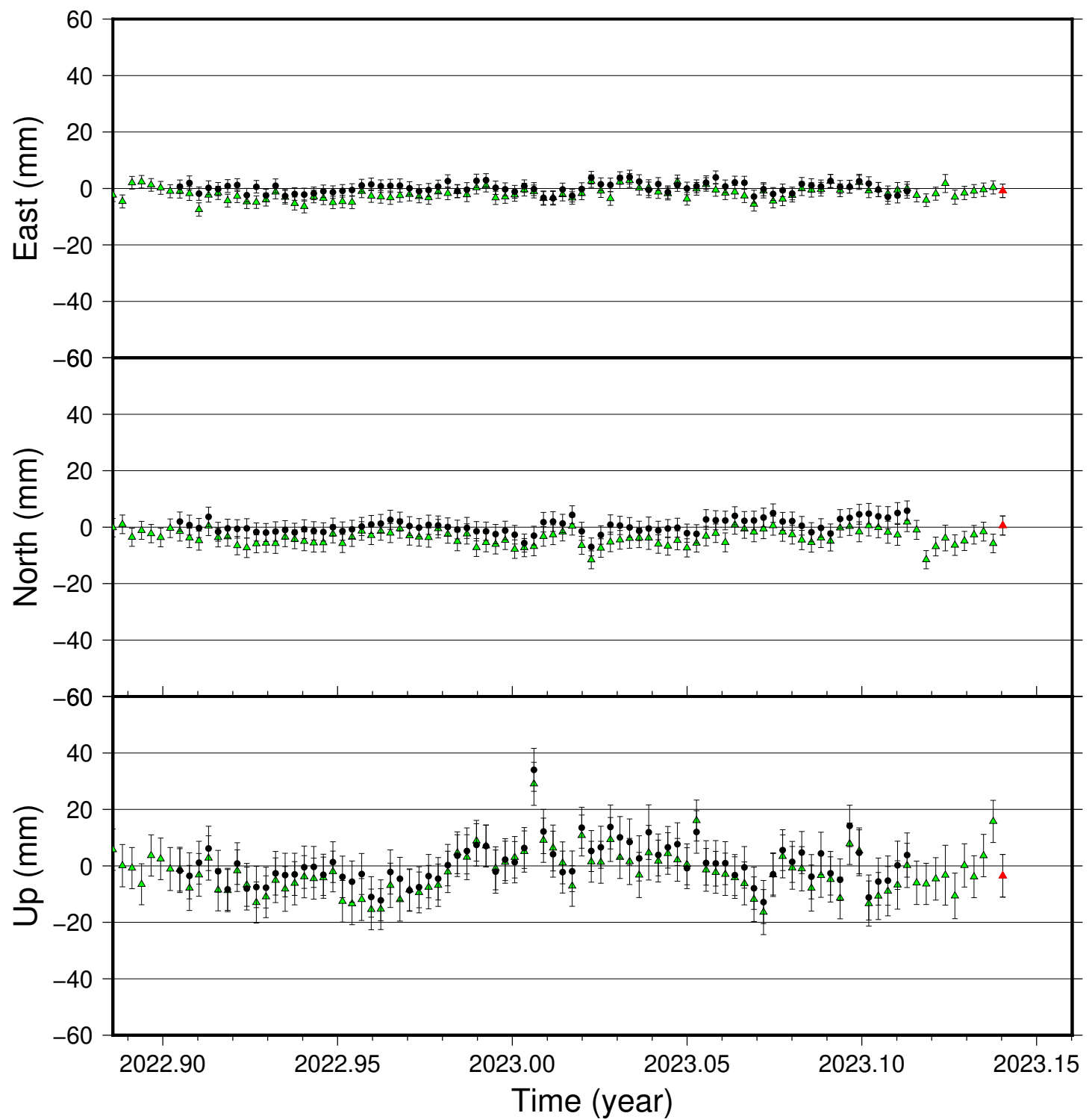
KOSK time series (IGS 2014), last 100 days
