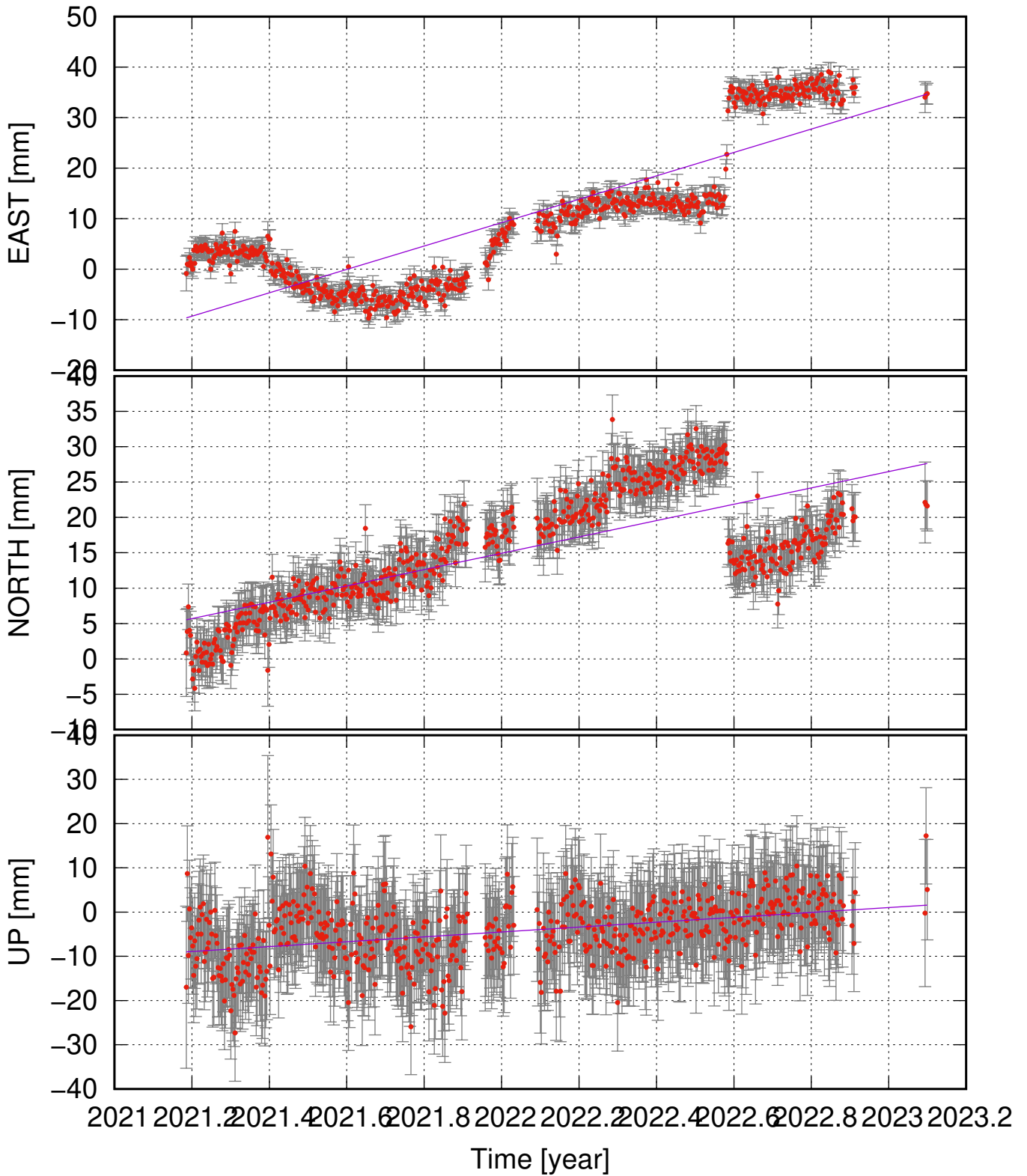
KLVC (63.91, -21.96) time series (ITRF 2014) v_e = 23.16 \pm 3.93 ; v_n = 11.56 \pm 2.81 ; v_u = 5.52 \pm 3.19 mm/yr
