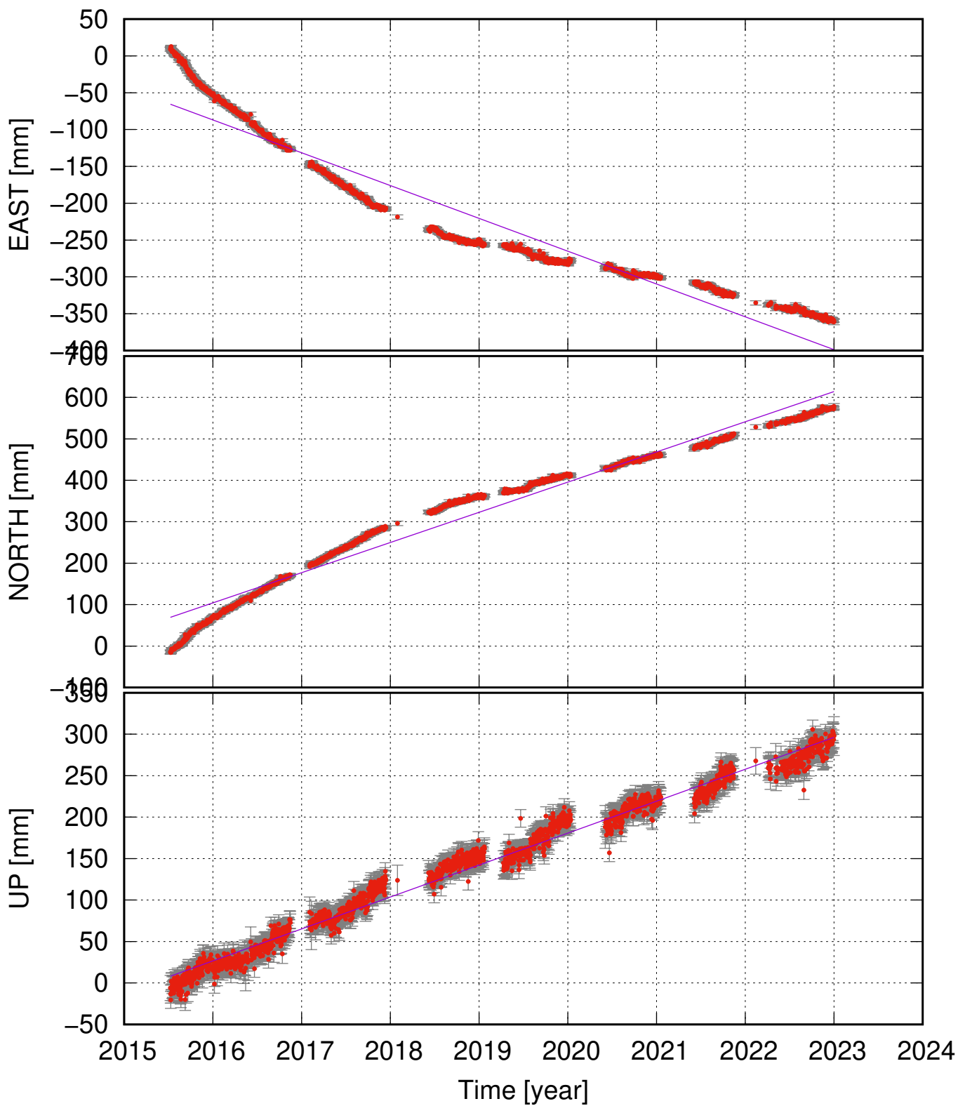
KISA (64.67, -17.56) time series (ITRF 2014) v_e = -44.54 \pm 3.92 ; v_n = 72.86 \pm 4.15 ; v_u = 38.50 \pm 1.49 mm/yr
