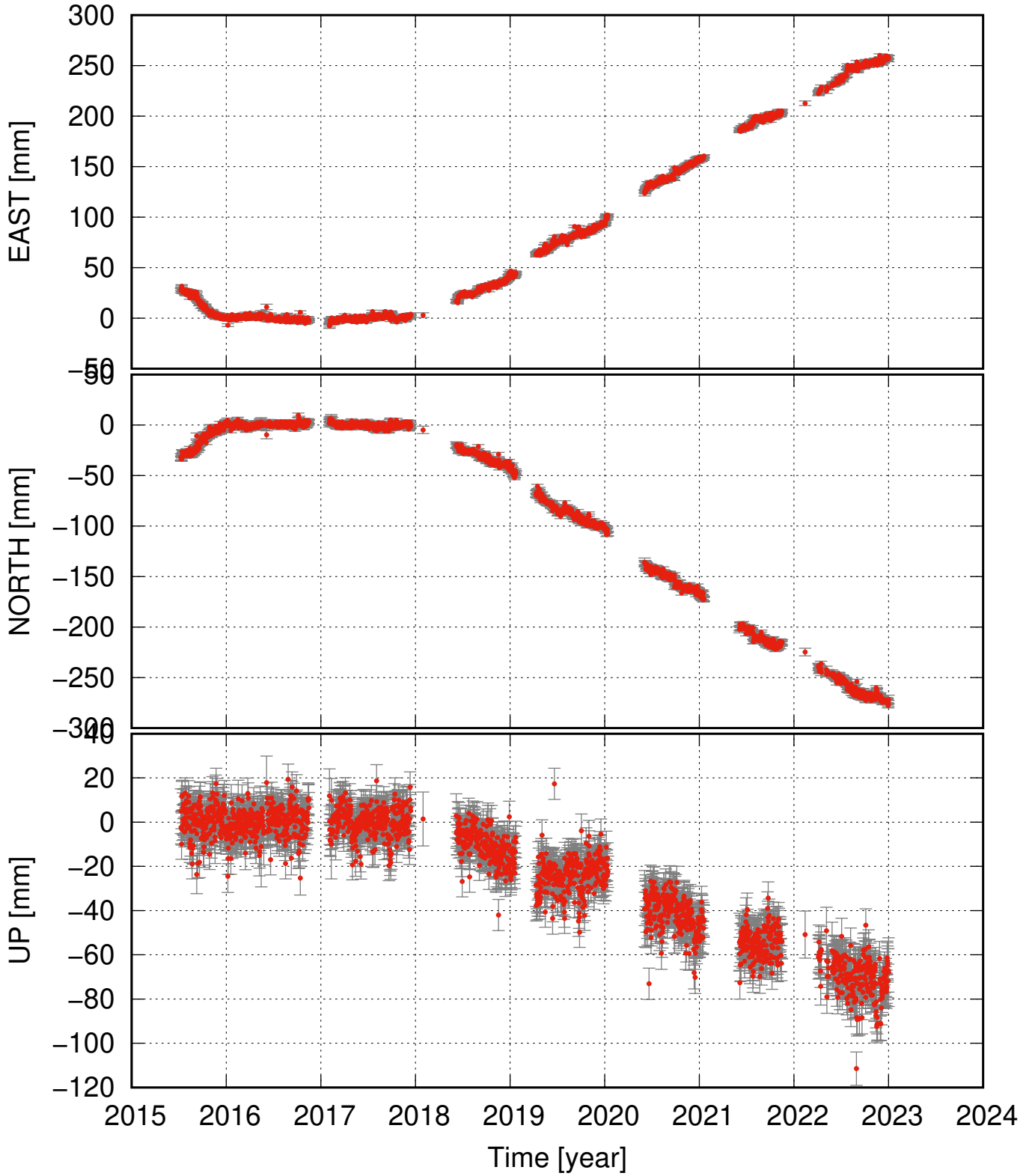
KISA detrended and seasonal signal removed
