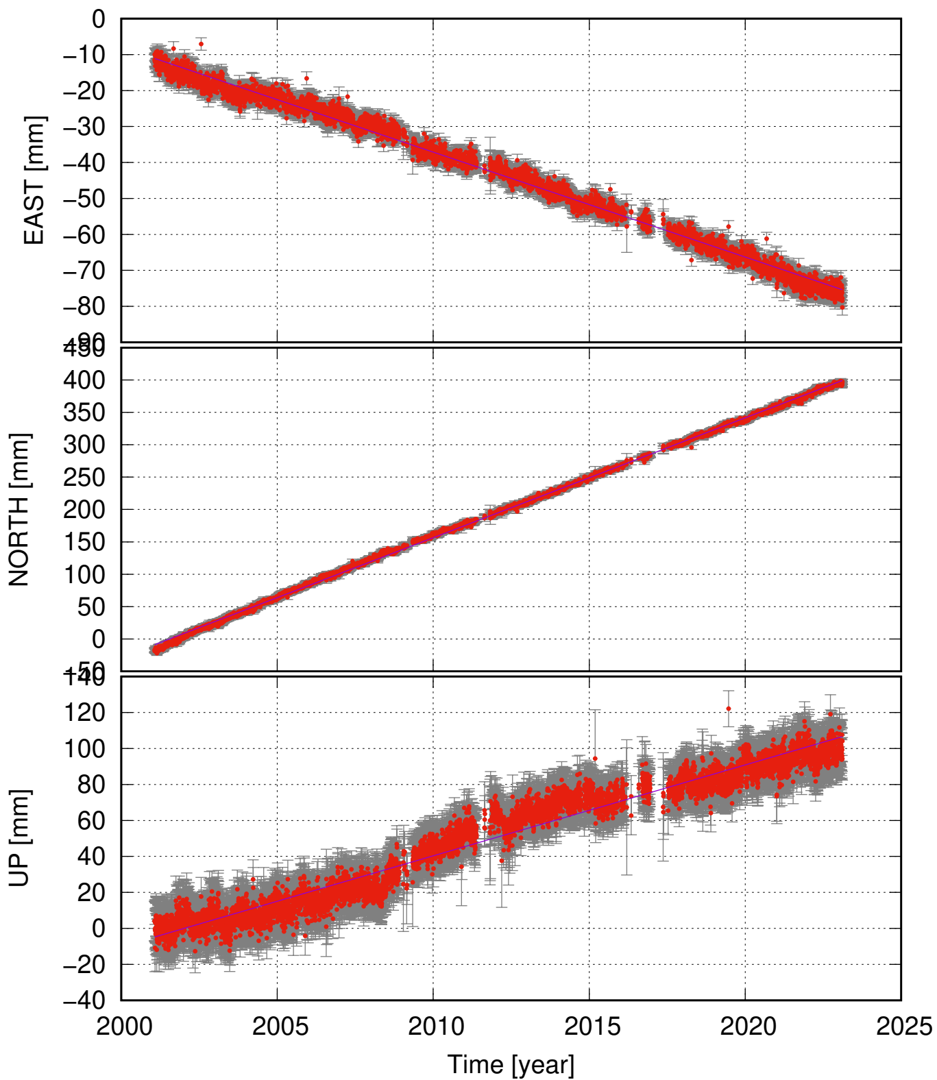
KIDJ (64.00, -20.77) time series (ITRF 2014) v_e = -2.92 \pm 0.08 ; v_n = 18.50 \pm 0.14 ; v_u = 5.05 \pm 0.32 mm/yr
