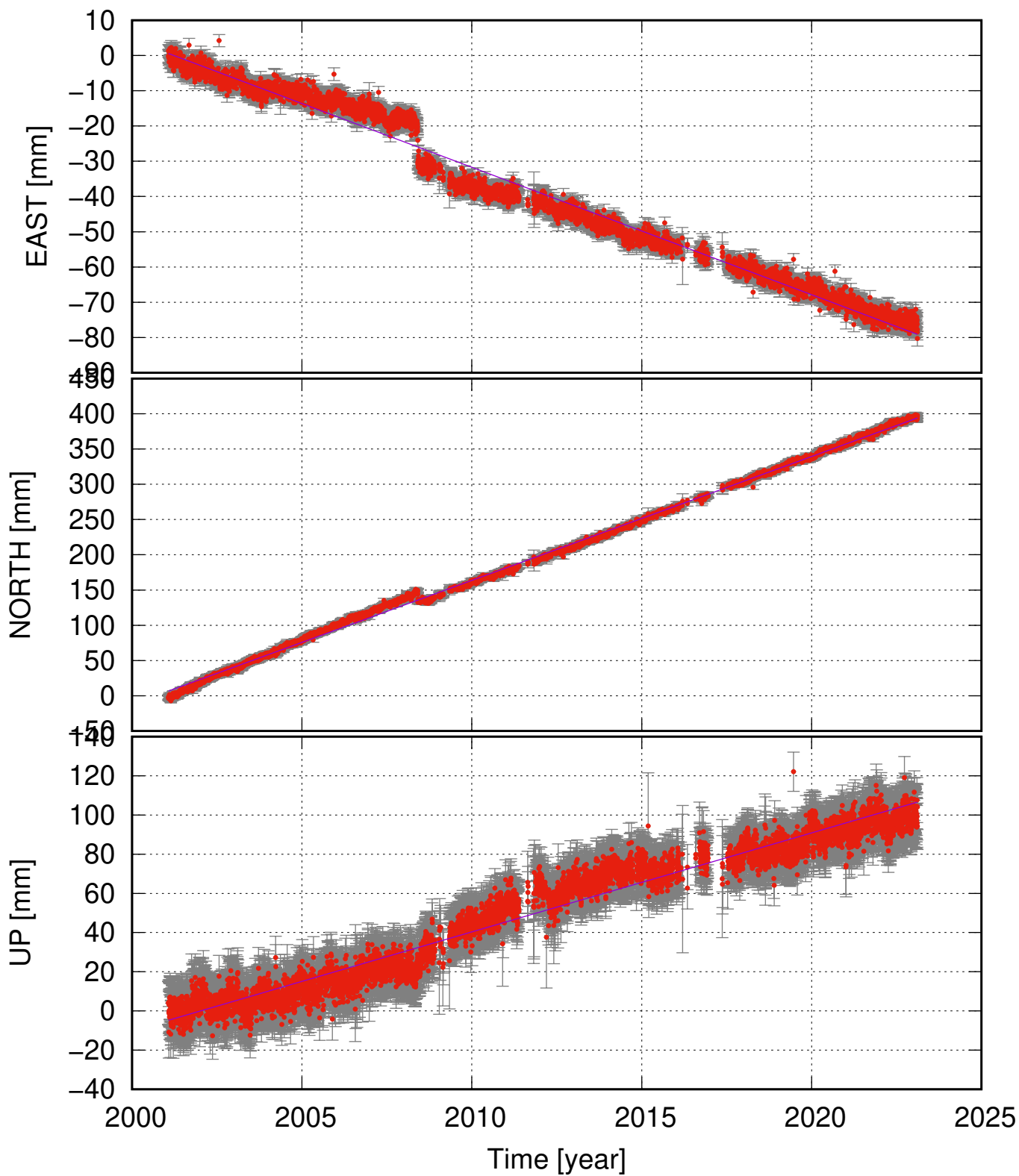
KIDJ (64.00, -20.77) time series (ITRF 2014) v_e = -3.61 \pm 0.15 ; v_n = 17.58 \pm 0.22 ; v_u = 5.05 \pm 0.32 mm/yr
