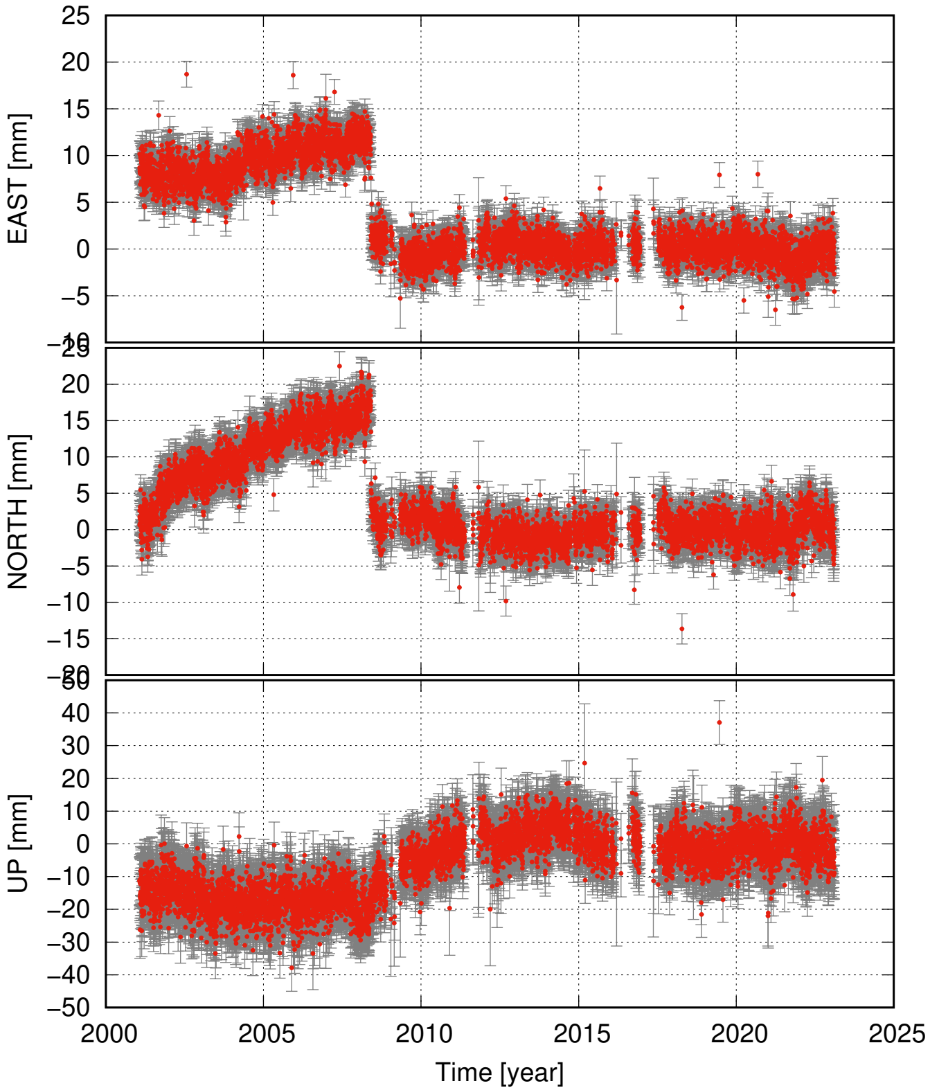
KIDJ detrended and seasonal signal removed
