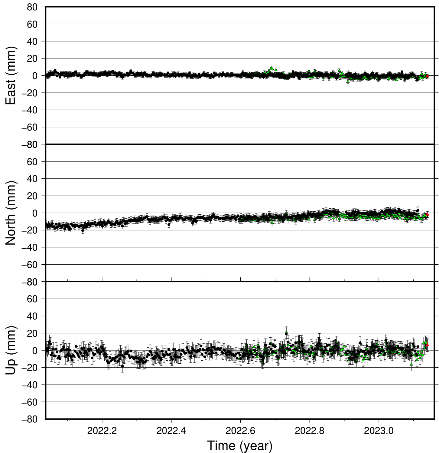
KIDJ time series (IGS 2014), last 400 days
