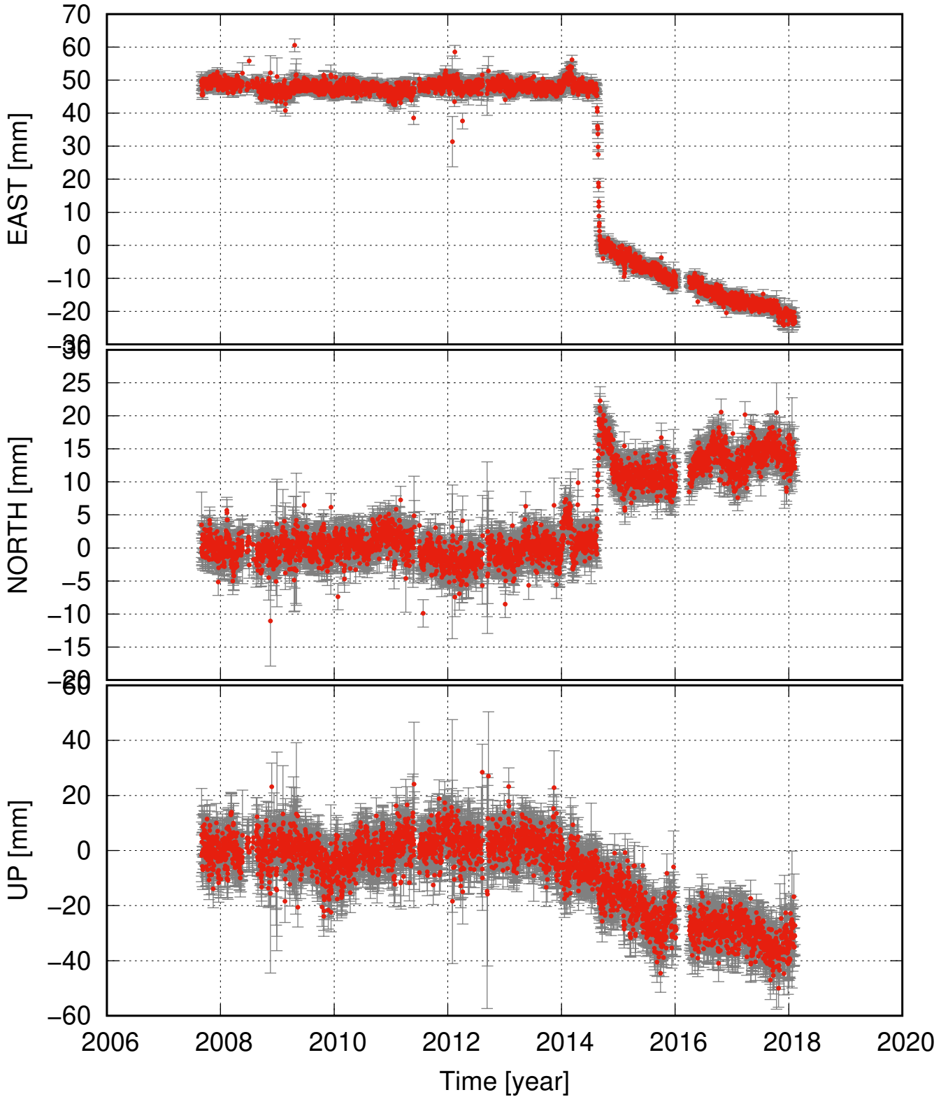
KIDC detrended and seasonal signal removed
