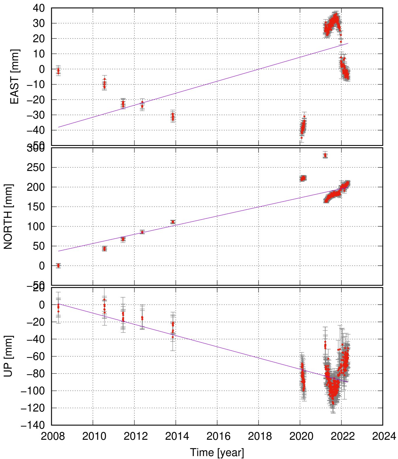
KAST (63.88, -22.32) time series (ITRF 2014) v_e = 3.92 \pm 1.58 ; v_n = 11.62 \pm 1.65 ; v_u = -6.52 \pm 1.16 mm/yr
