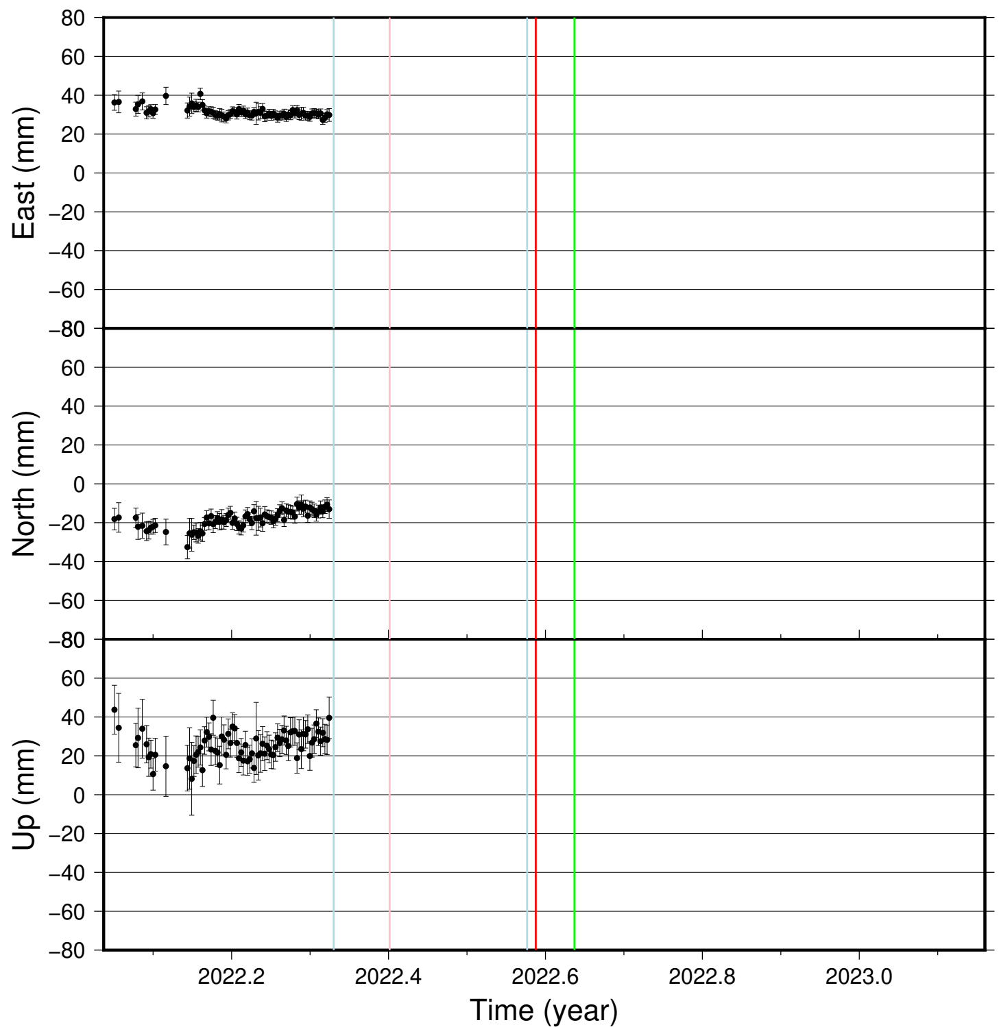
KAST time series (IGS 2014), last 400 days
