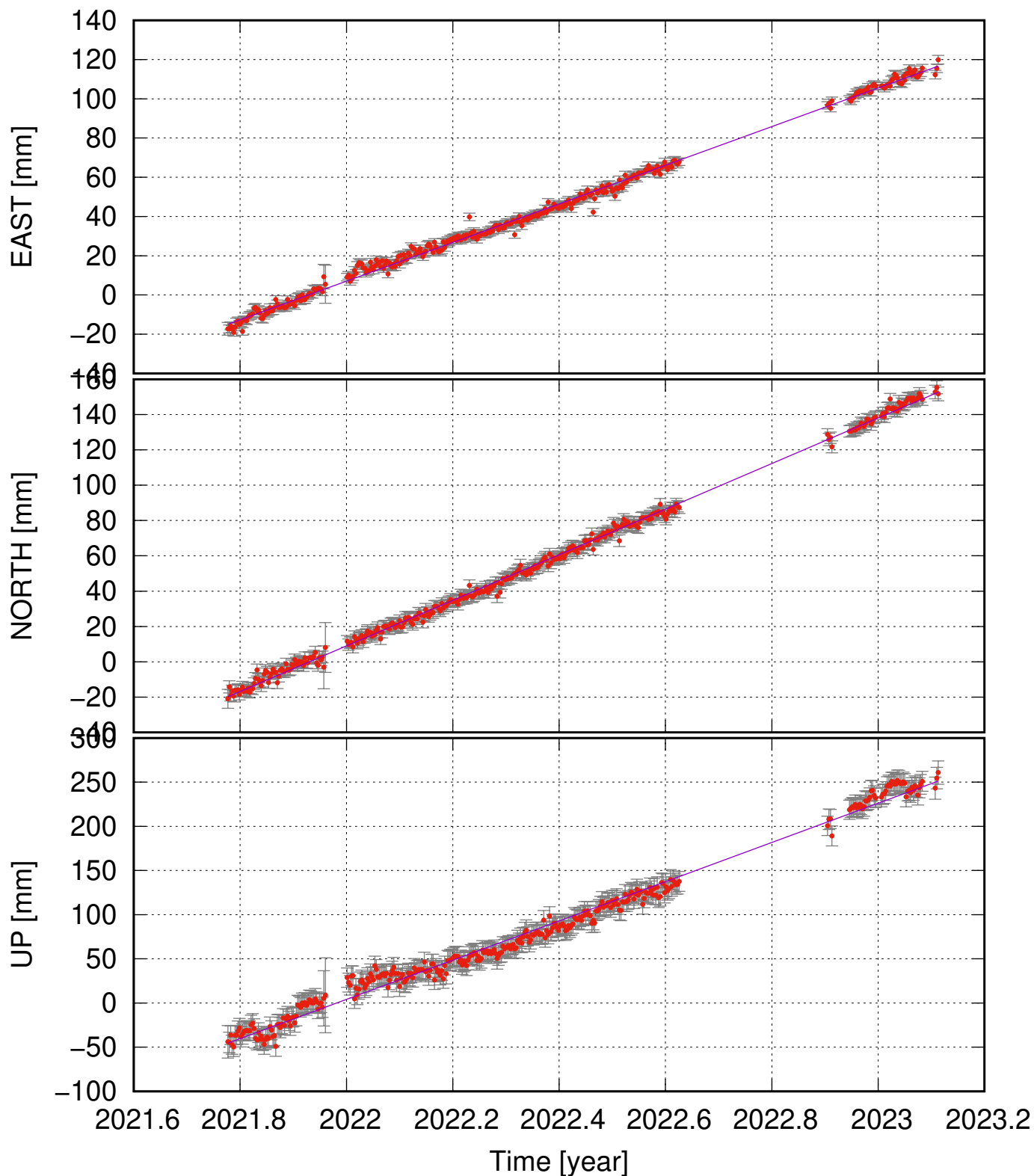
KASC (65.06, -16.76) time series (ITRF 2014) v_e = 98.44 \pm 1.66 ; v_n = 129.10 \pm 1.66 ; v_u = 222.01 \pm 6.69 mm/yr
