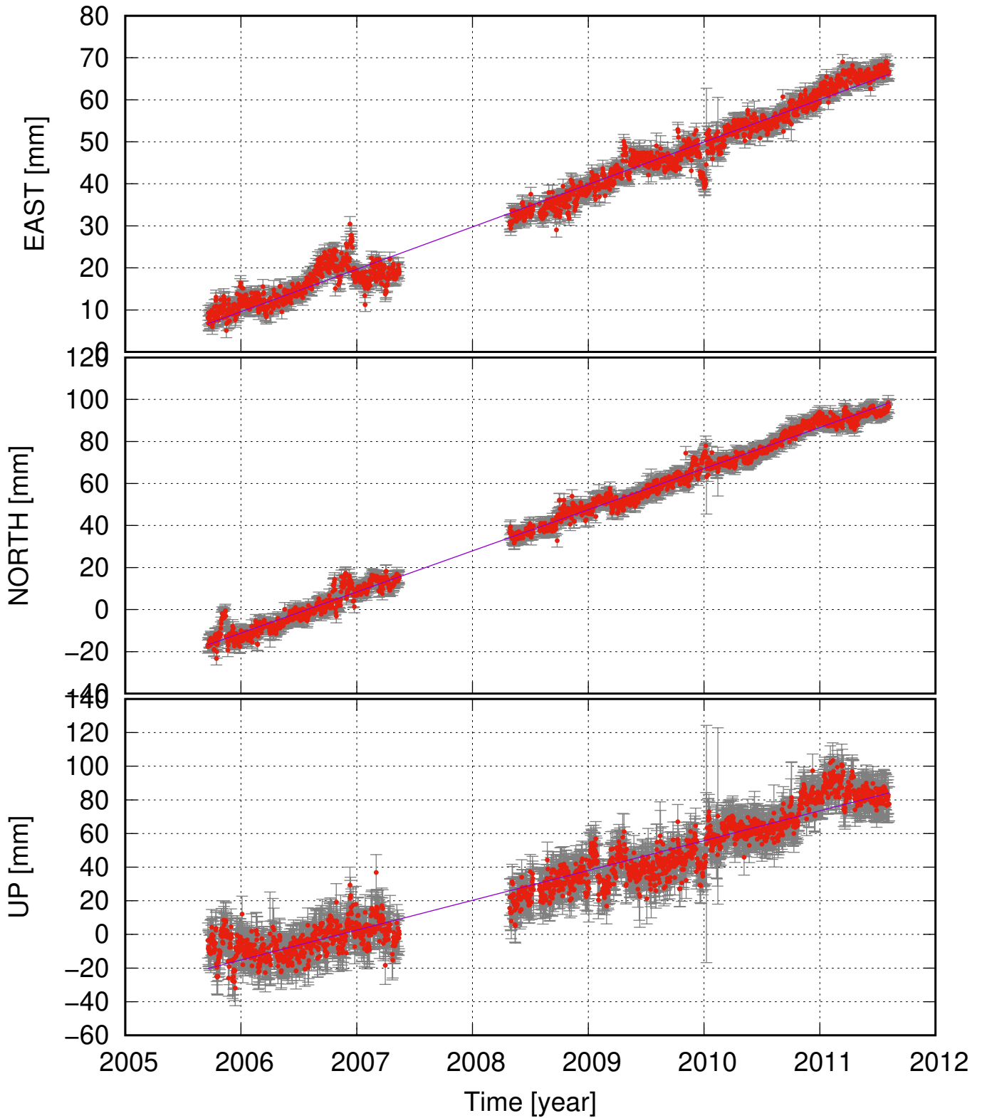
KARV (64.93, -15.84) time series (ITRF 2014) v_e = 10.09 \pm 0.43 ; v_n = 19.56 \pm 0.49 ; v_u = 17.74 \pm 1.48 mm/yr
