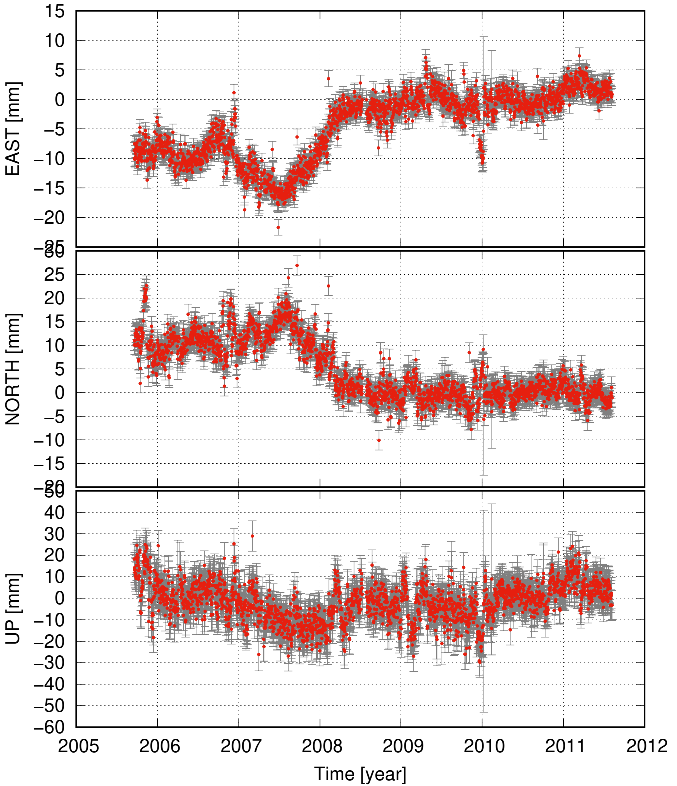
KARV detrended and seasonal signal removed
