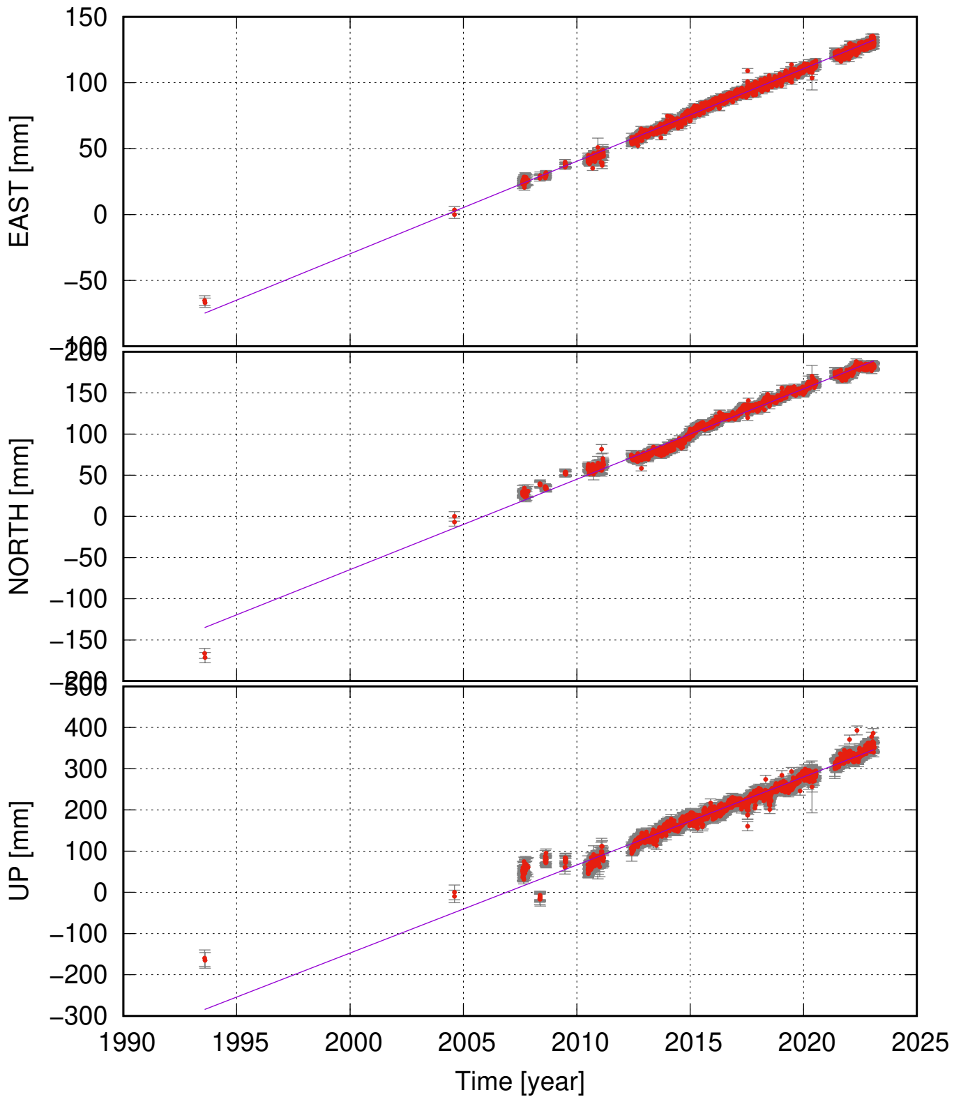
KALF (63.95, -17.69) time series (ITRF 2014) v_e = 7.02 \pm 0.06 ; v_n = 10.97 \pm 0.15 ; v_u = 21.35 \pm 0.36 mm/yr
