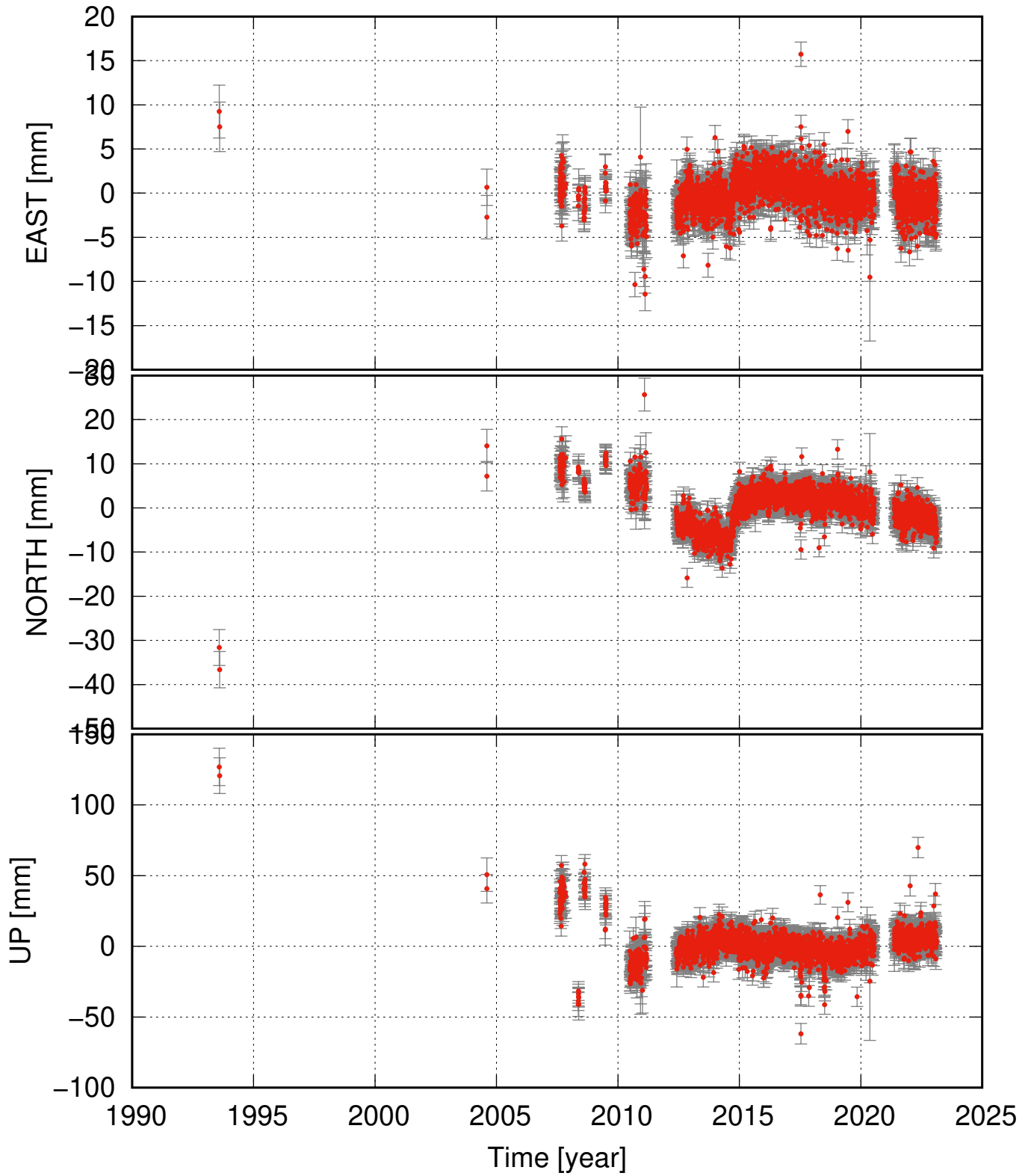
KALF detrended and seasonal signal removed
