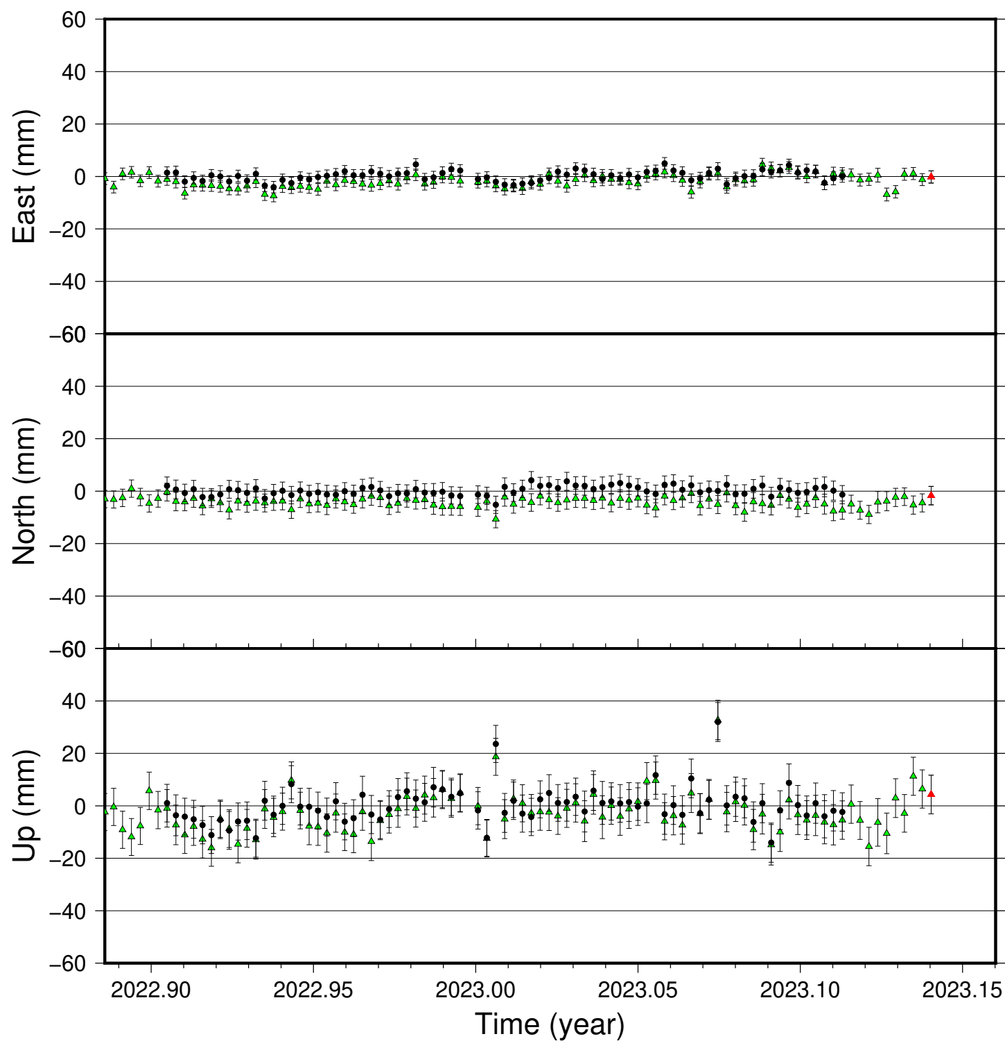
KALF time series (IGS 2014), last 100 days
