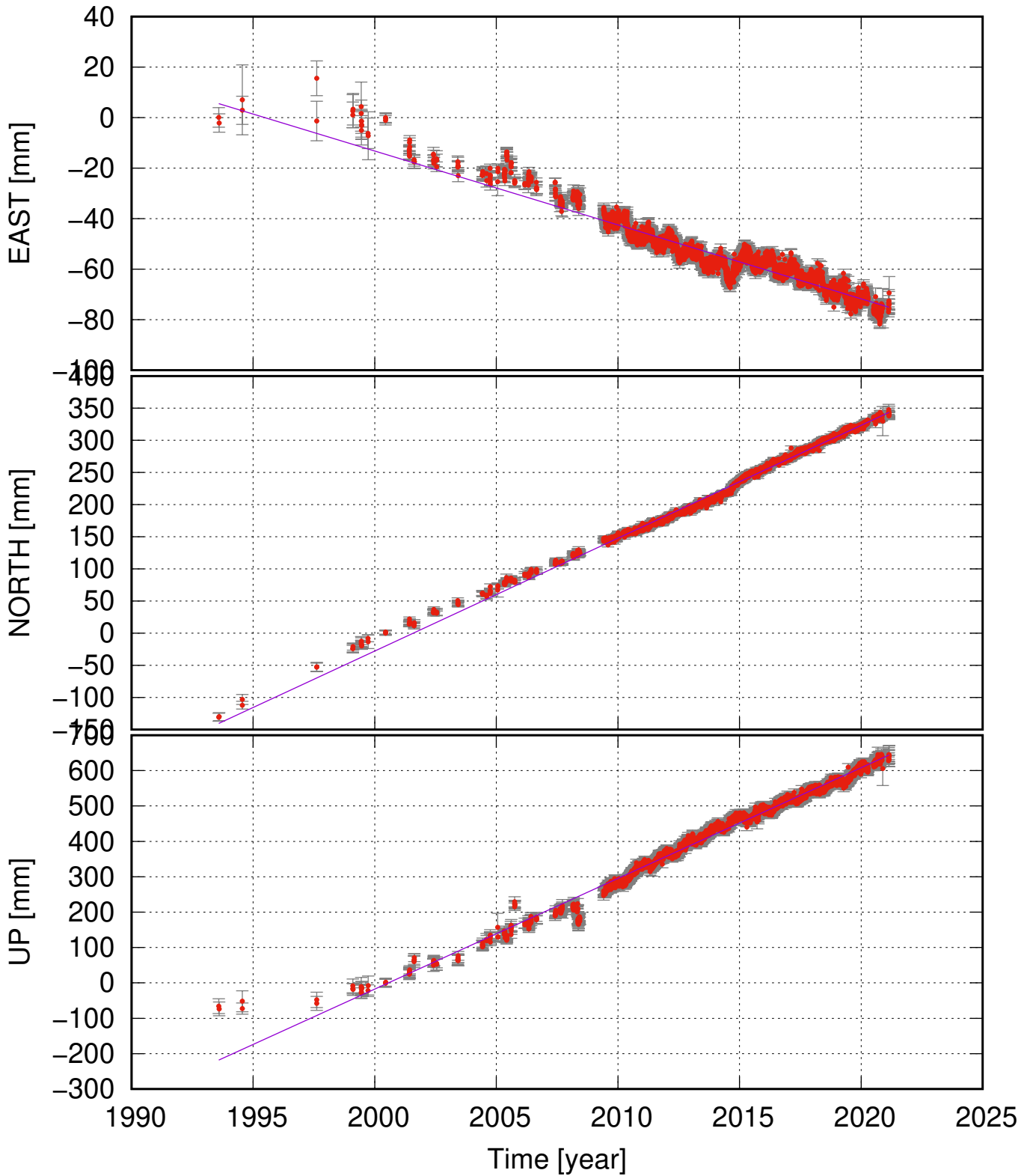
JOKU (64.31, -18.24) time series (ITRF 2014) v_e = -2.92 \pm 0.12 ; v_n = 17.56 \pm 0.19 ; v_u = 31.28 \pm 0.49 mm/yr
