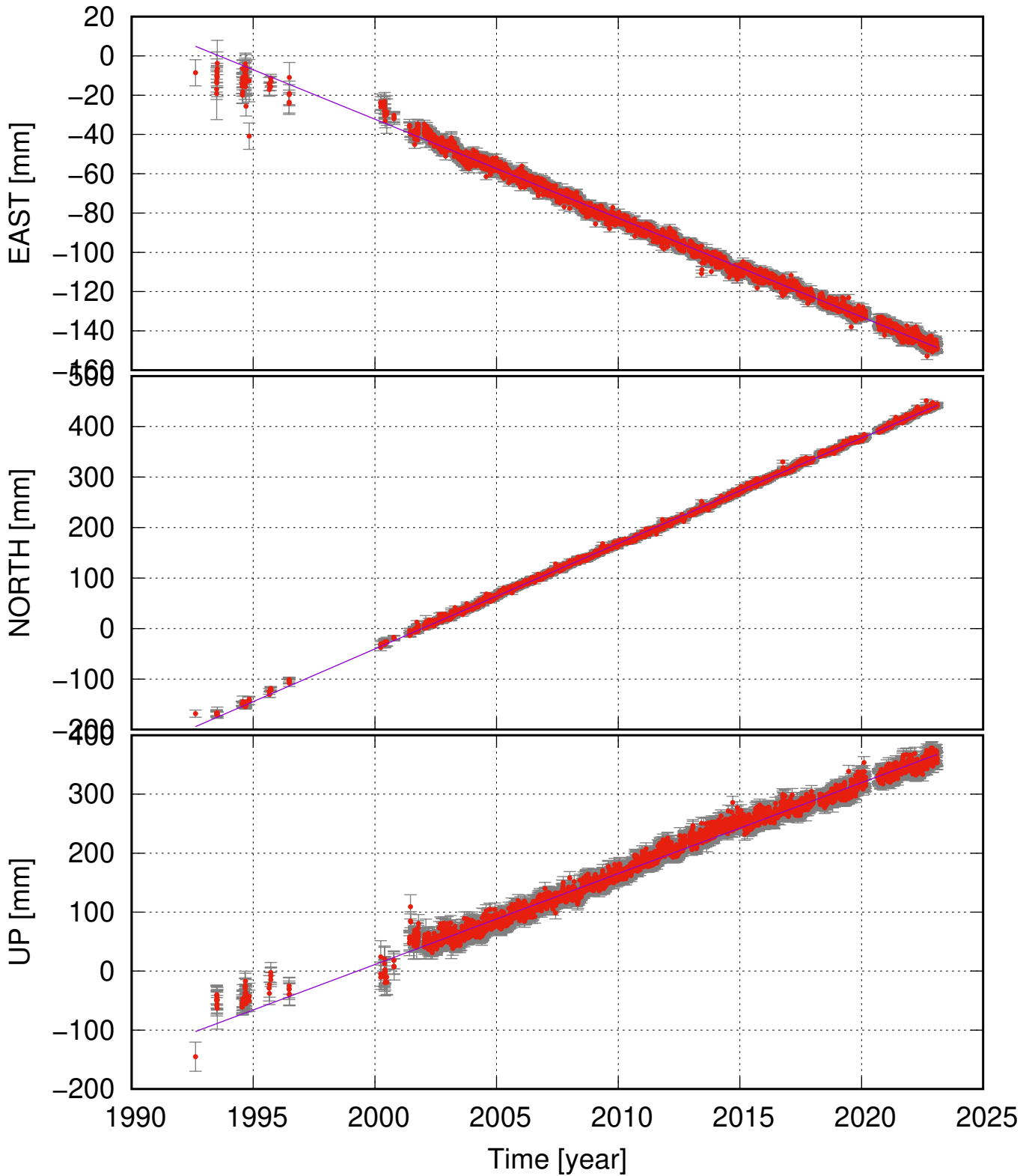
ISAK (64.12, -19.75) time series (ITRF 2014) v_e = -5.03 \pm 0.07 ; v_n = 20.85 \pm 0.10 ; v_u = 15.41 \pm 0.30 mm/yr
