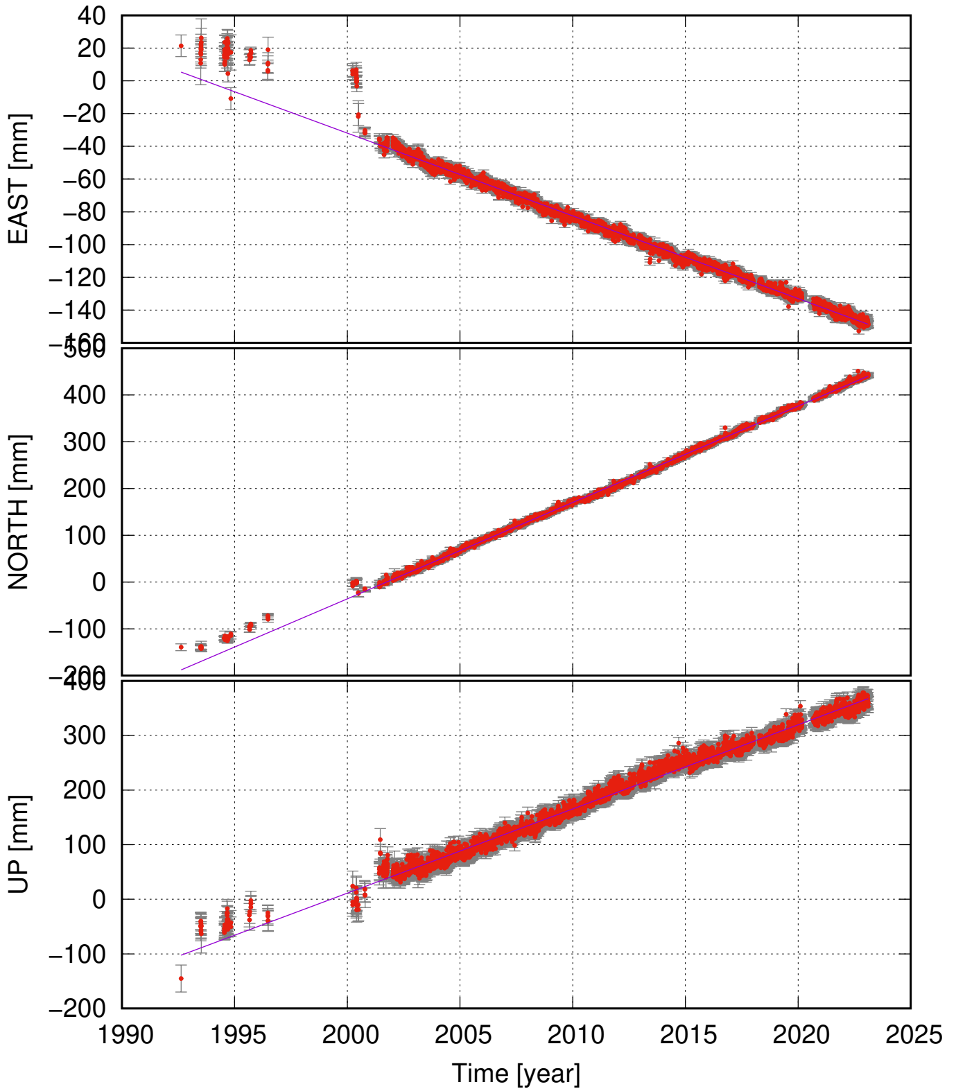
ISAK (64.12, -19.75) time series (ITRF 2014) v_e = -5.05 \pm 0.10 ; v_n = 20.60 \pm 0.14 ; v_u = 15.41 \pm 0.30 mm/yr
