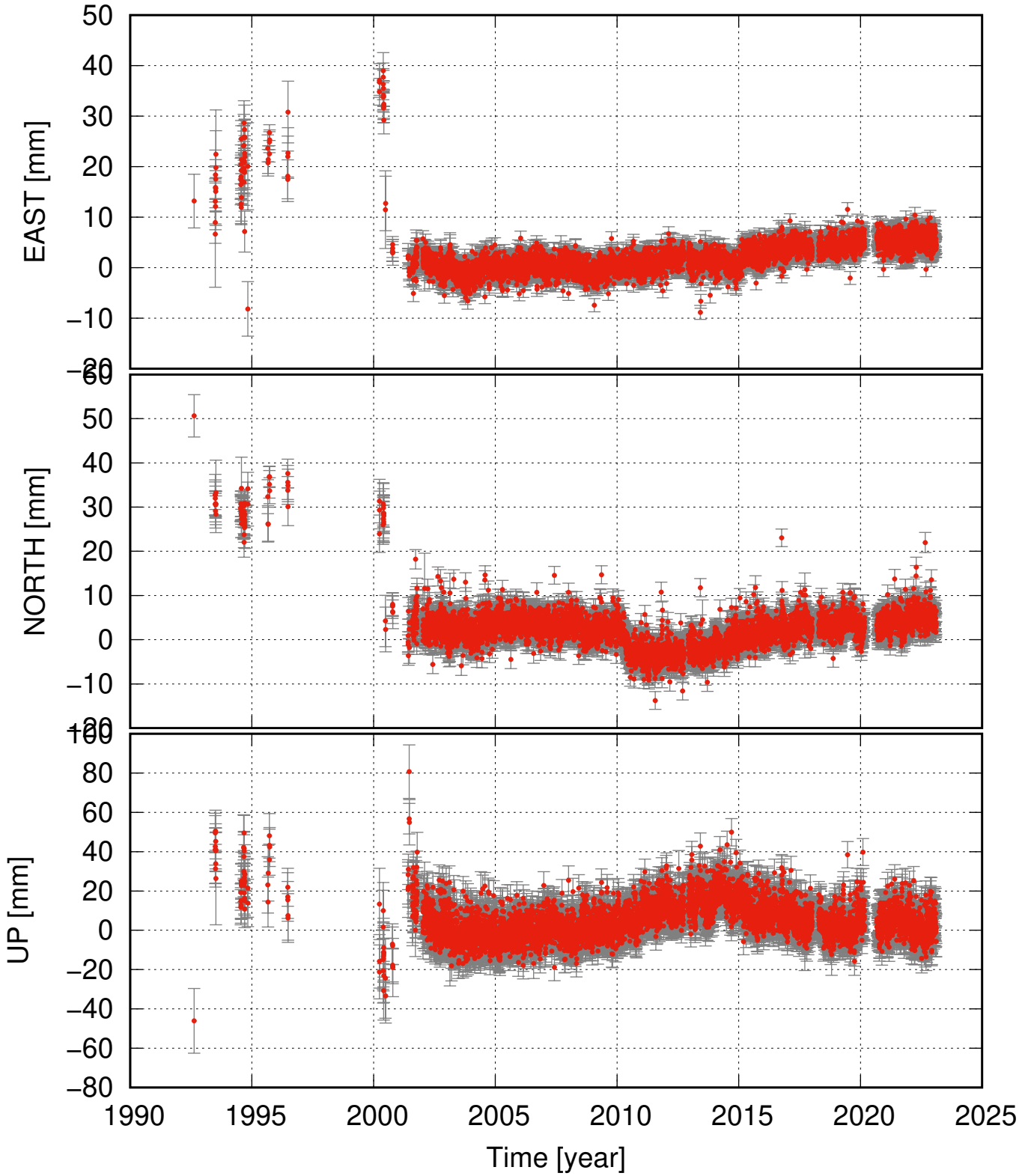
ISAK detrended and seasonal signal removed
