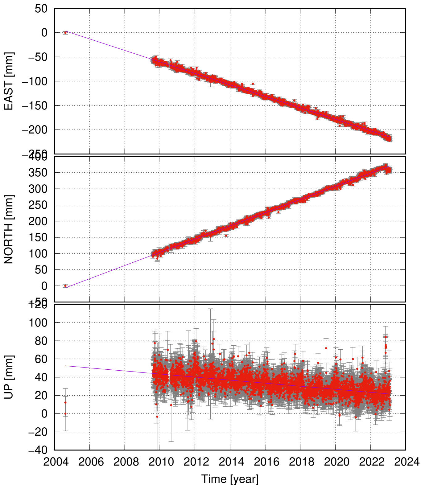
ISAF (66.07, -23.12) time series (ITRF 2014) ve = -11.82 \pm 0.12 ; vn = 20.39 \pm 0.19 ; vu = -1.67 \pm 0.43 mm/yr
