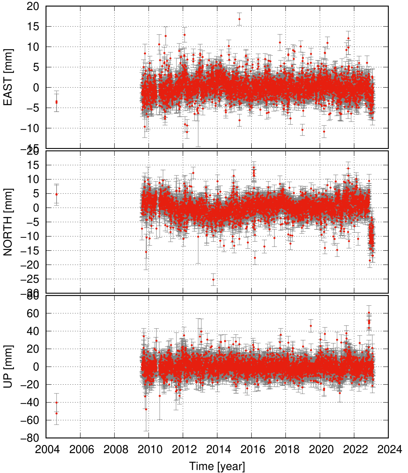
ISAF detrended and seasonal signal removed
