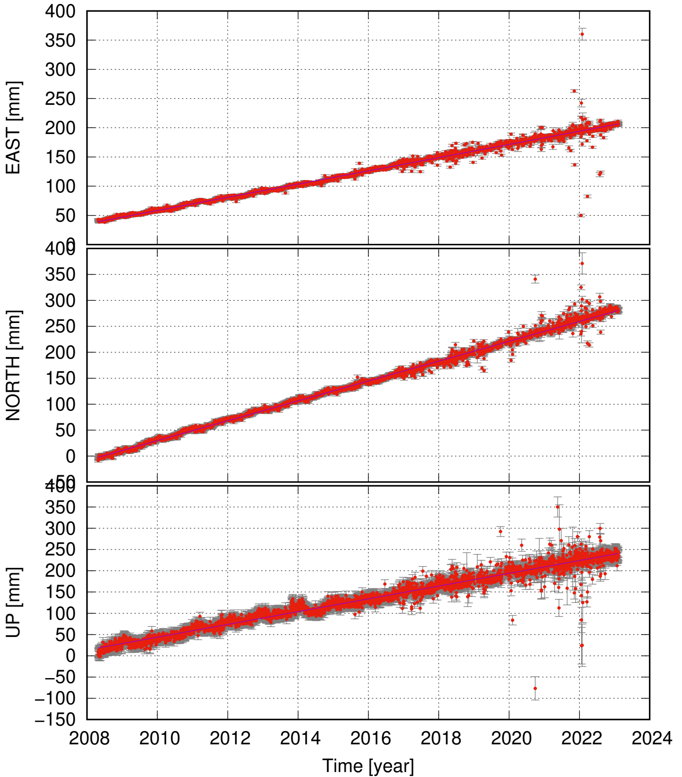
INTA (64.94, -15.78) time series (ITRF 2014) v_e = 11.31 \pm 0.33 ; v_n = 19.12 \pm 0.33 ; v_u = 15.03 \pm 0.79 mm/yr
