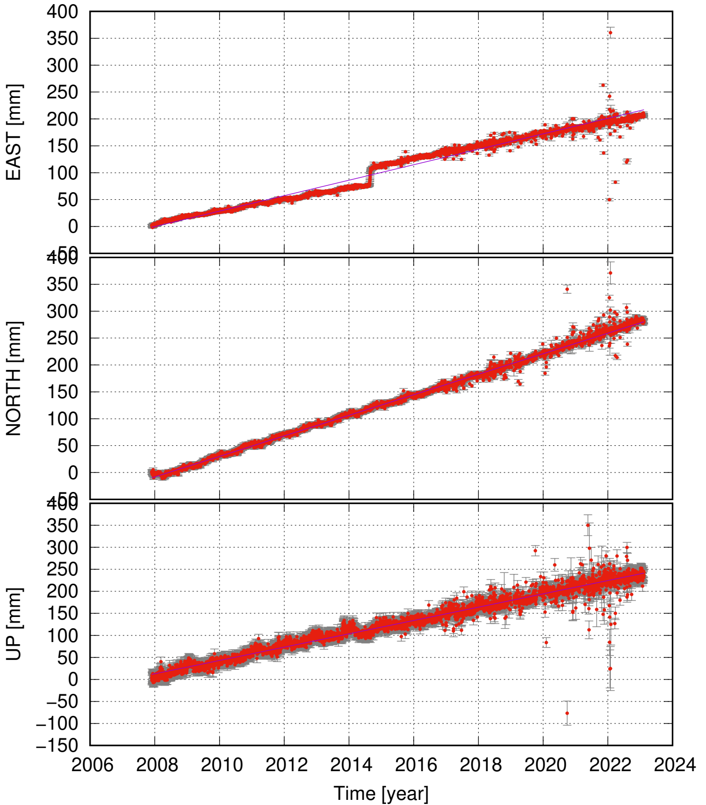
INTA (64.94, -15.78) time series (ITRF 2014) v_e = 14.36 \pm 0.62 ; v_n = 19.08 \pm 0.32 ; v_u = 15.12 \pm 0.77 mm/yr
