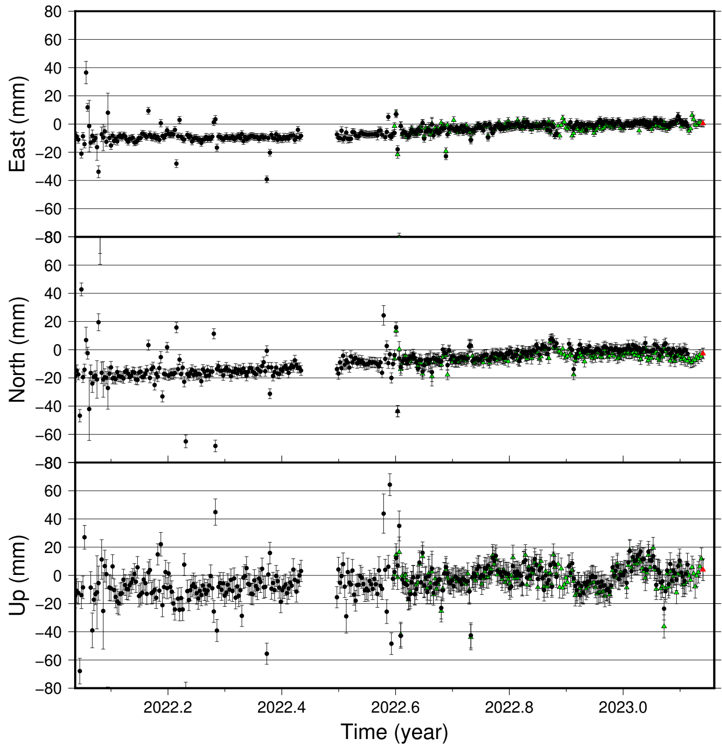
INTA time series (IGS 2014), last 400 days
