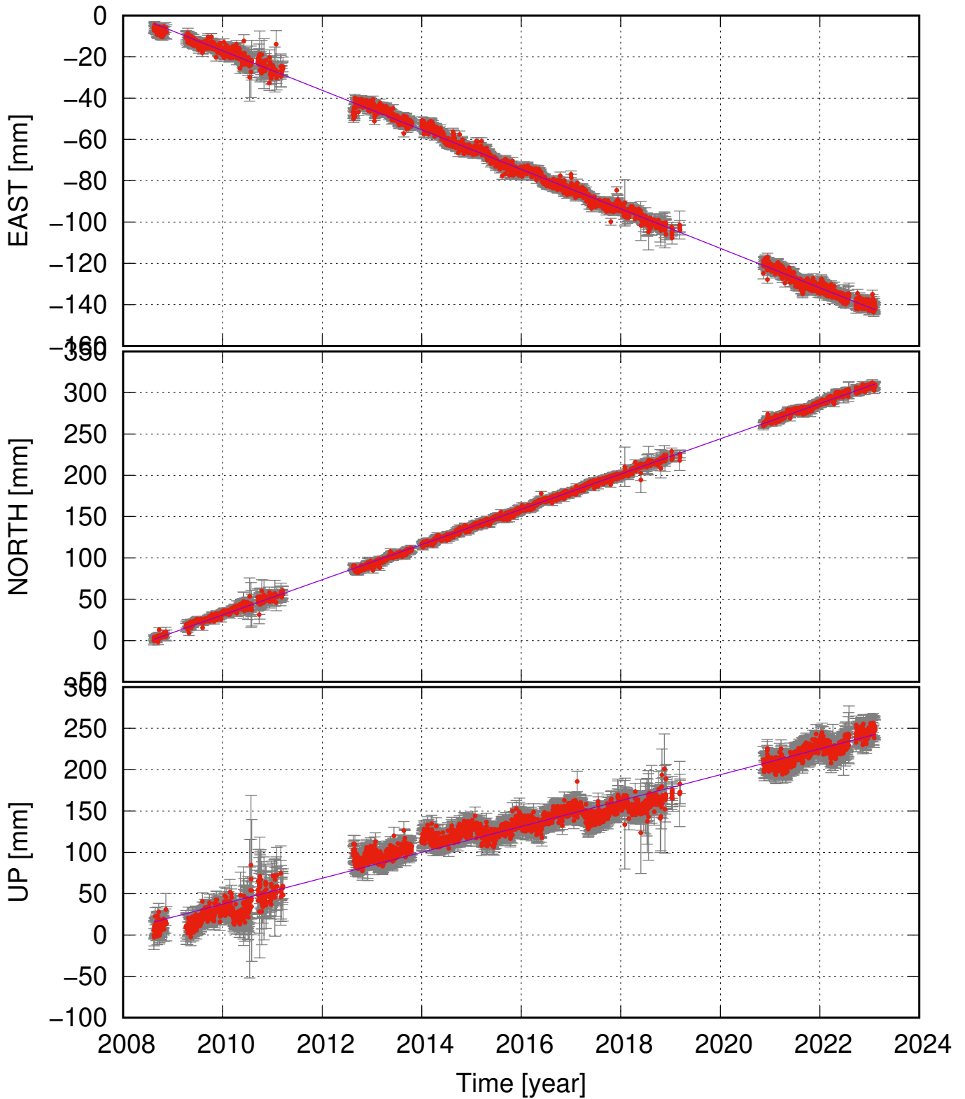
INSK (64.68, -19.53) time series (ITRF 2014) v_e = -9.56 \pm 0.12 ; v_n = 21.31 \pm 0.15 ; v_u = 15.66 \pm 0.71 mm/yr
