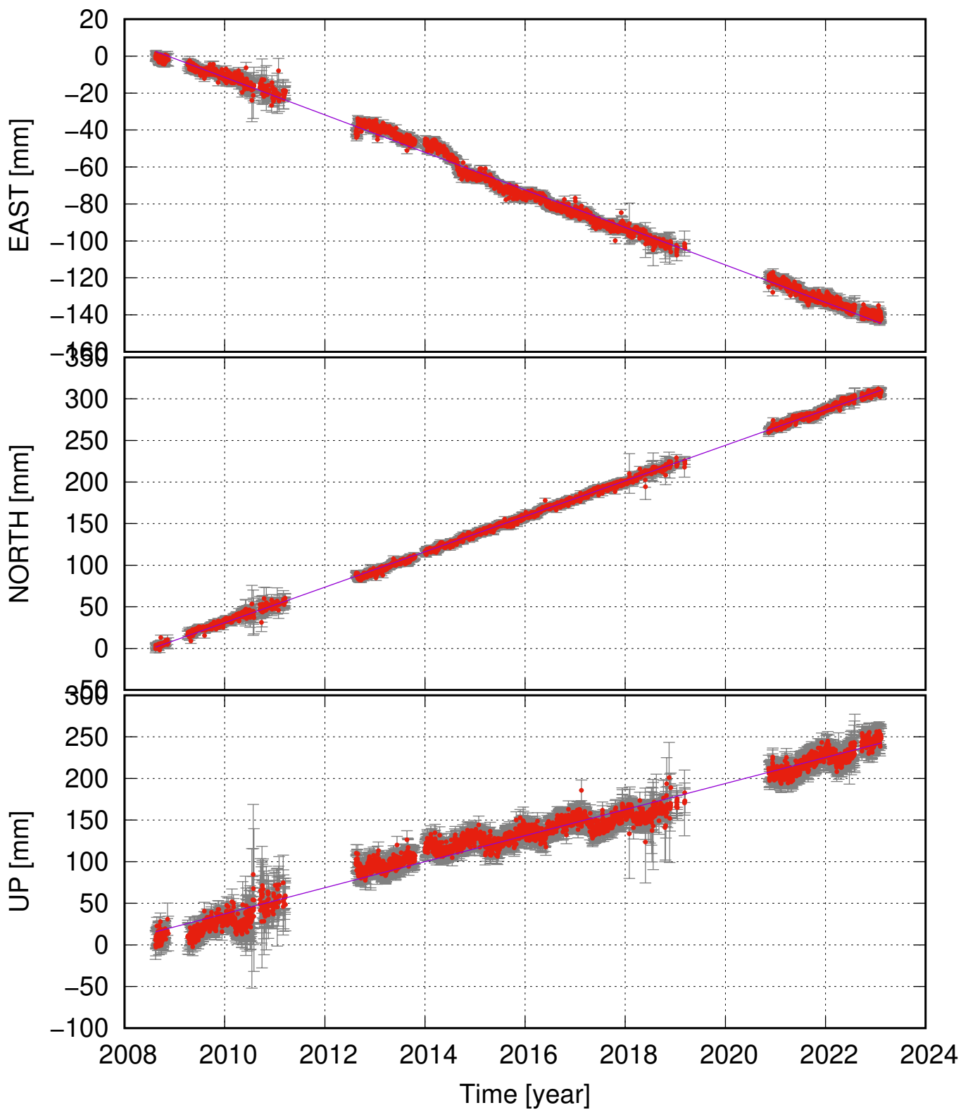
INSK (64.68, -19.53) time series (ITRF 2014) ve = -10.15 \pm 0.19 ; vn = 21.31 \pm 0.15 ; vu = 15.66 \pm 0.71 mm/yr
