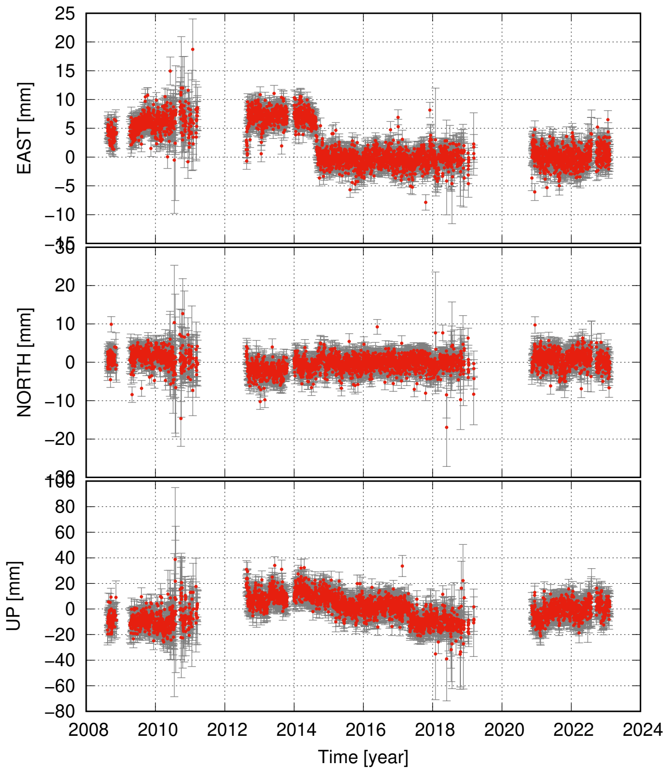
INSK detrended and seasonal signal removed
