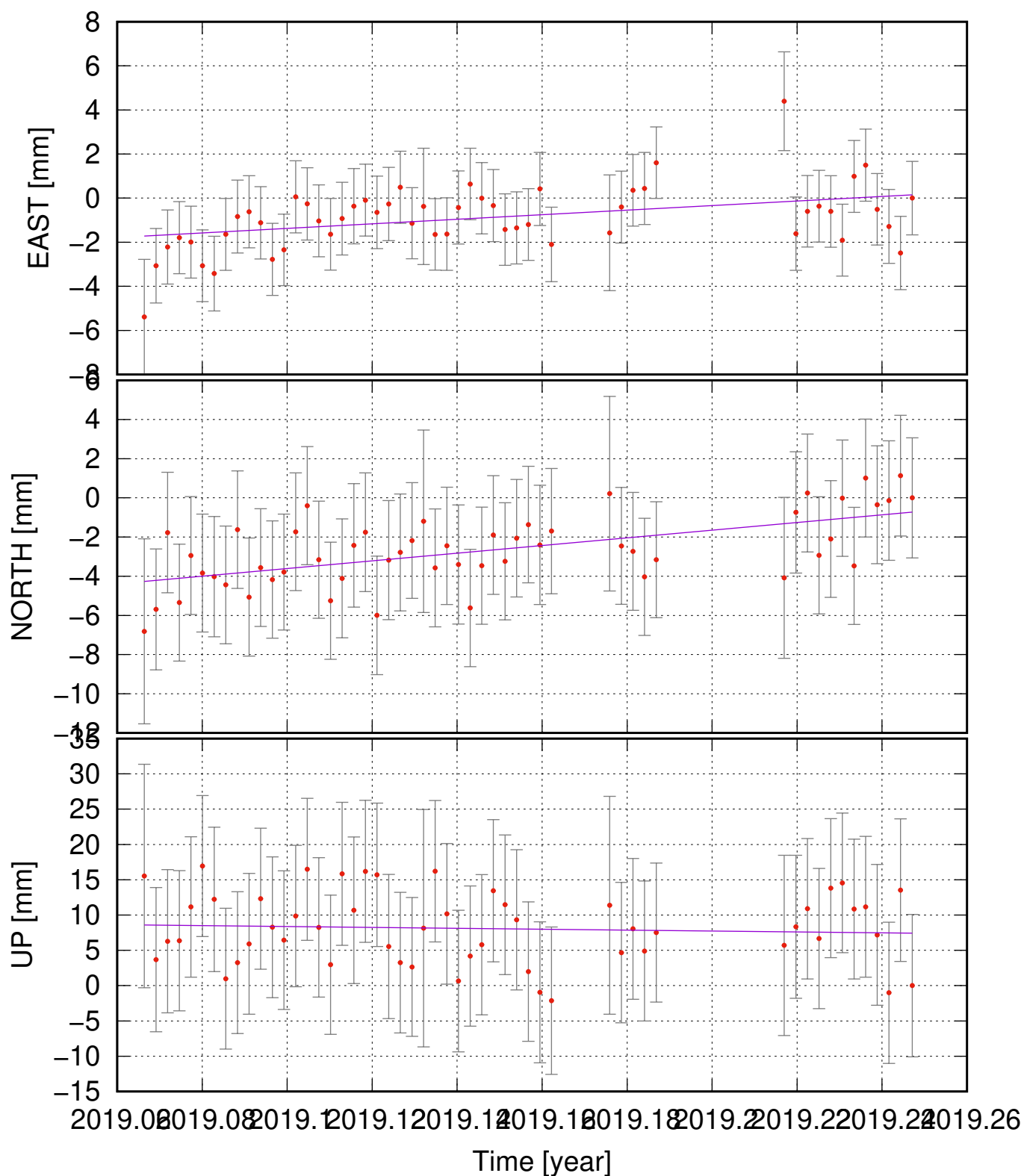
INGC (63.80, -16.65) time series (ITRF 2014) ve = 10.36 \pm 7.35 ; vn = 19.55 \pm 8.17 ; vu = -6.26 \pm 28.50 mm/yr
