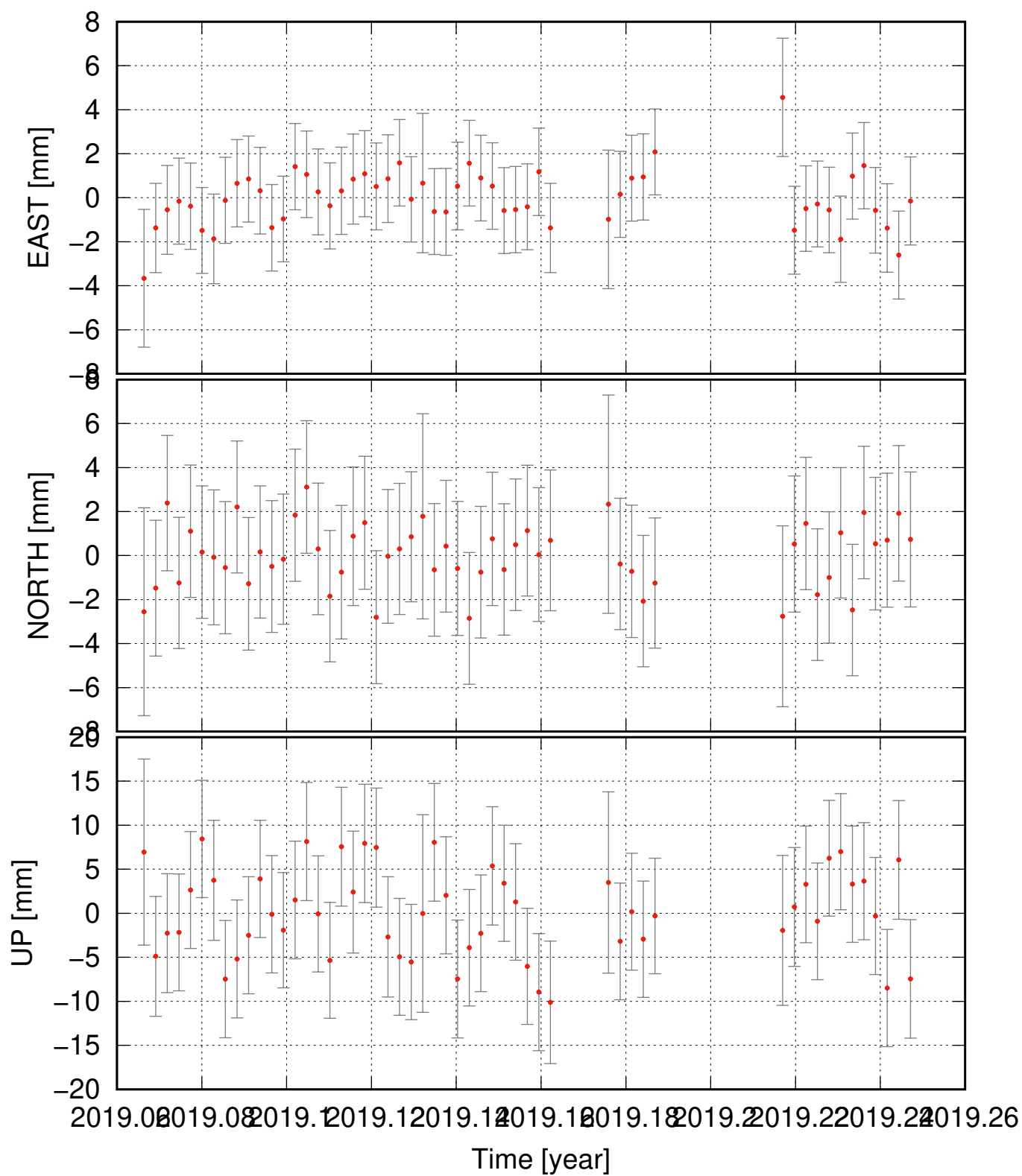
INGC residual time series (some major events removed as well)
