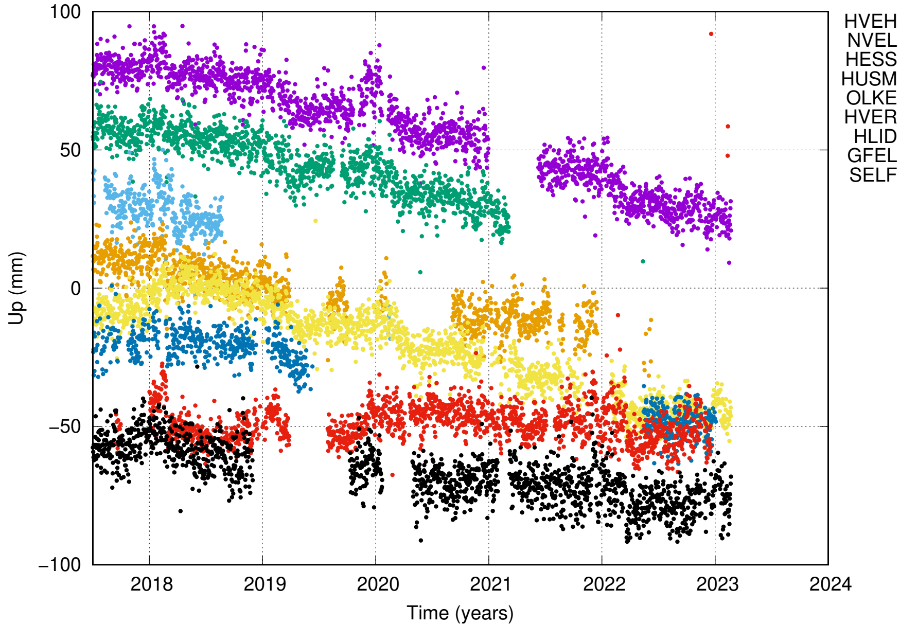
Hengill stations vertical component in ITRF2008 since 2017.5
