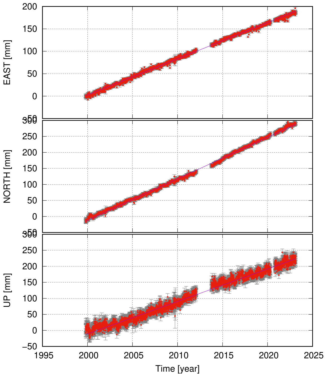
HVOL (63.53, -18.85) time series (ITRF 2014) v_e = 8.08 \pm 0.10 ; v_n = 12.98 \pm 0.18 ; v_u = 10.14 \pm 0.38 mm/yr
