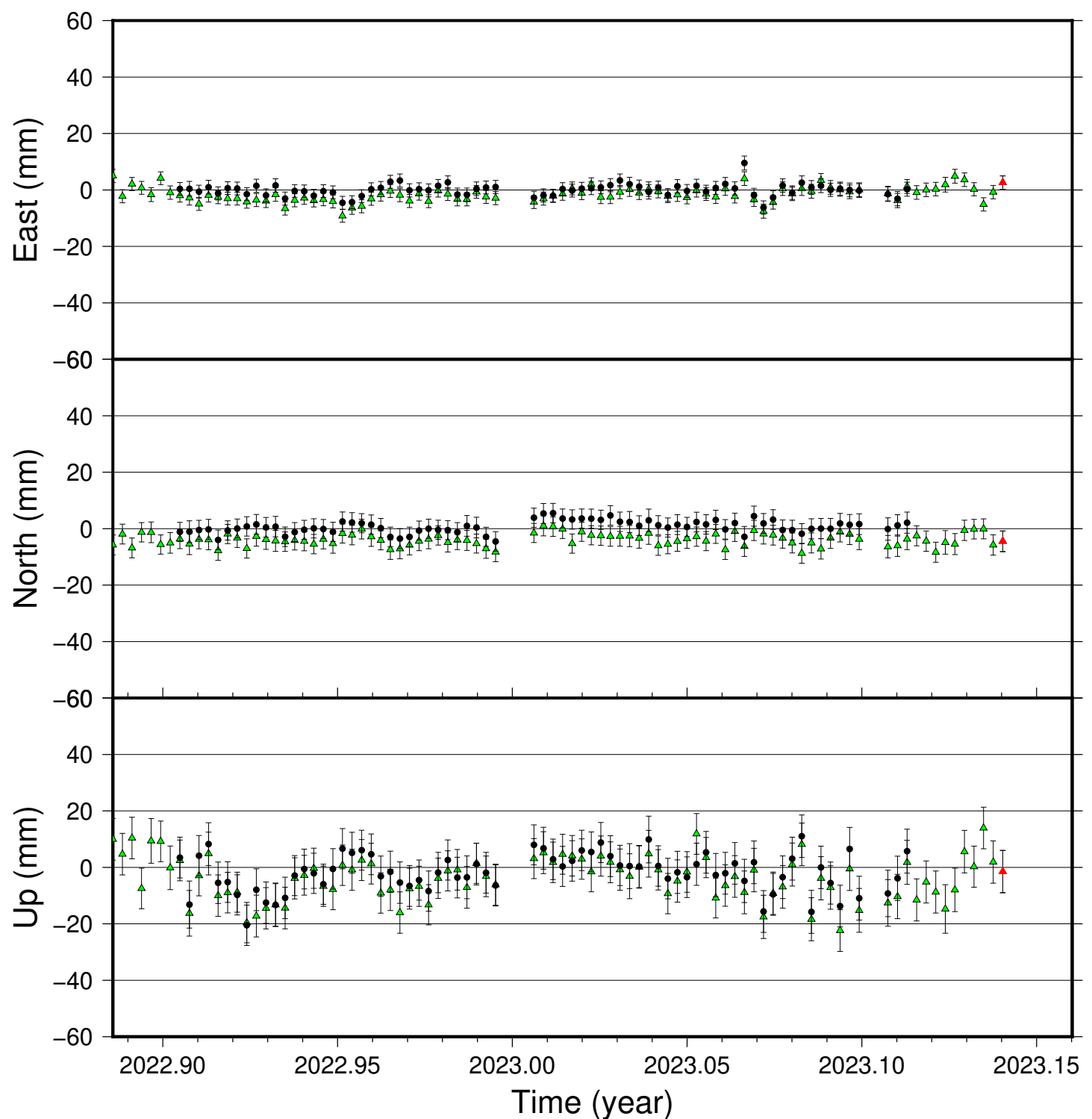
HVOL time series (IGS 2014), last 100 days
