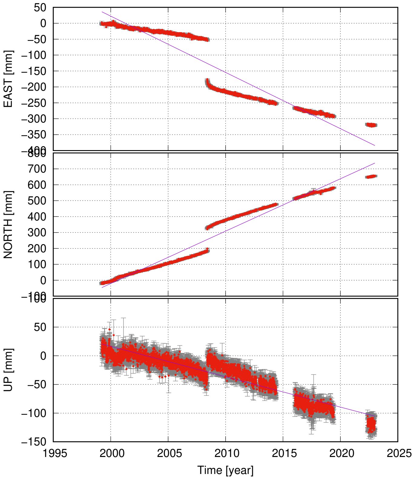
HVER (64.02, -21.18) time series (ITRF 2014) v_e = -17.68 \pm 1.73 ; v_n = 32.90 \pm 1.89 ; v_u = -5.30 \pm 0.48 mm/yr
