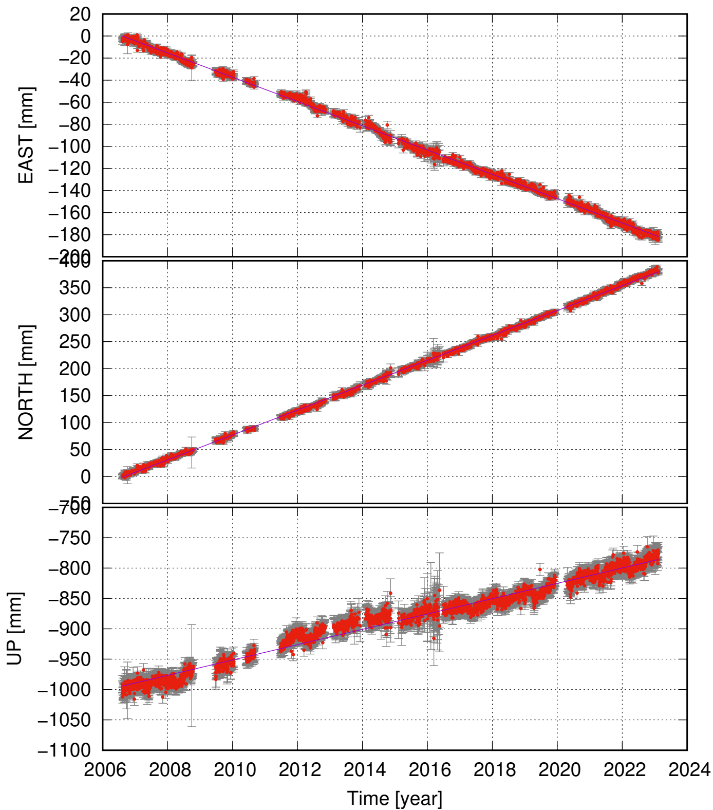
HVEL (64.87, -19.56) time series (ITRF 2014) v_e = -11.01 \pm 0.13 ; v_n = 23.06 \pm 0.17 ; v_u = 12.62 \pm 0.58 mm/yr
