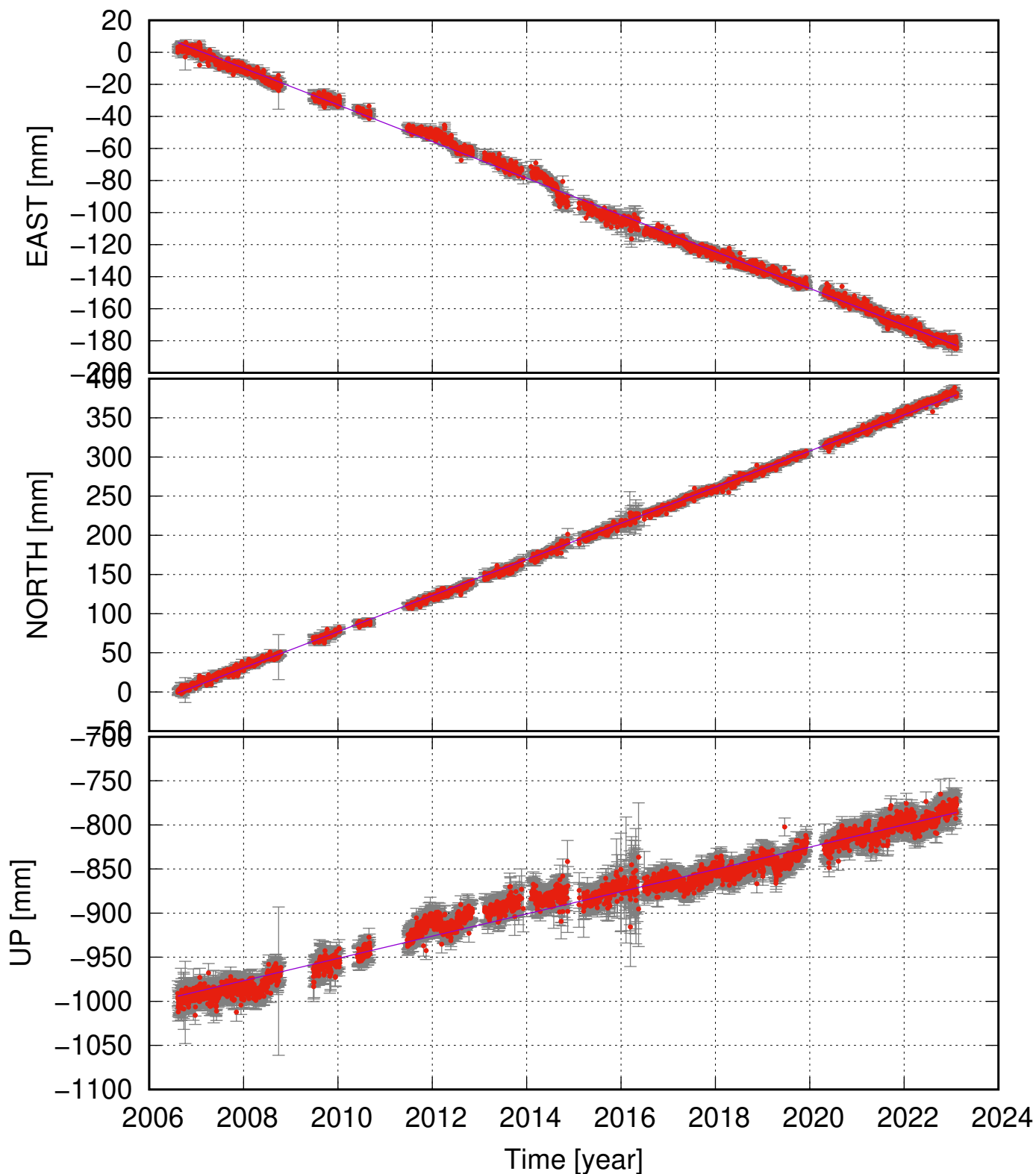
HVEL (64.87, -19.56) time series (ITRF 2014) v_e = -11.45 \pm 0.17 ; v_n = 23.06 \pm 0.17 ; v_u = 12.62 \pm 0.58 mm/yr
